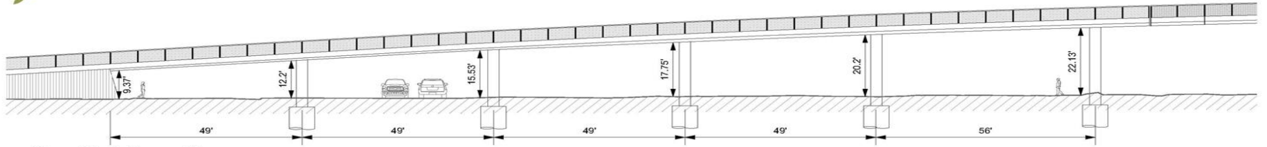
South Elevation
