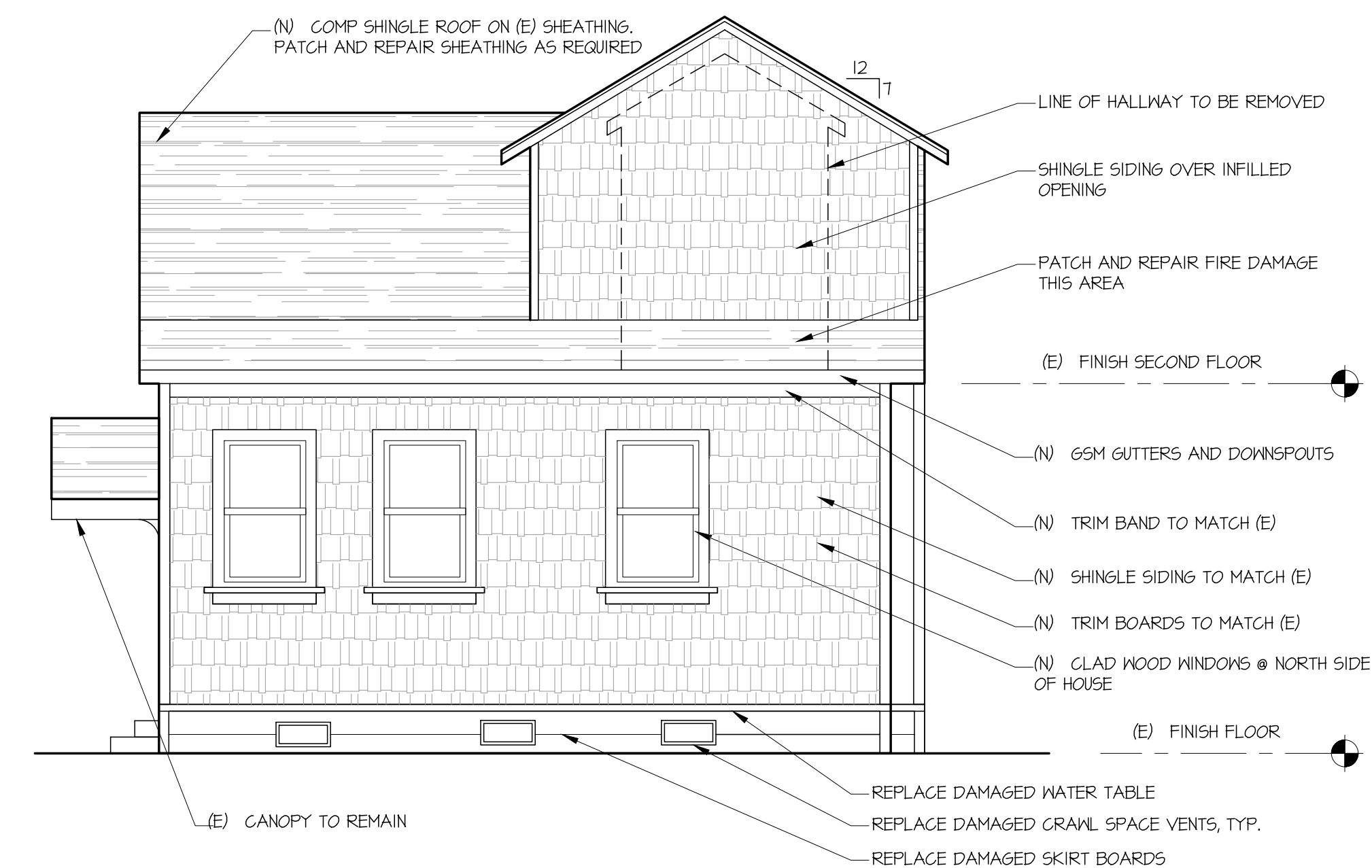
4 PROPOSED NORTH ELEVATION 1/4"=1'-0"
