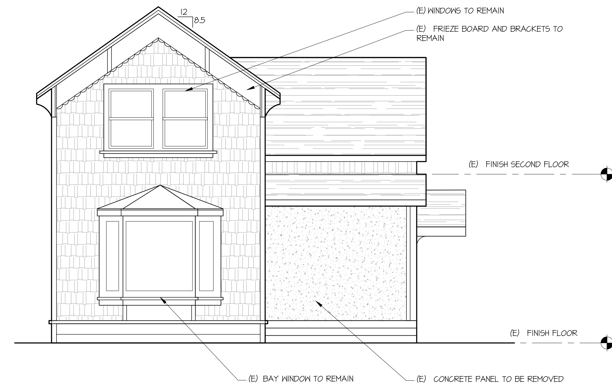
2 EXISTING SOUTH ELEVATION 1/4"=1'-0"
