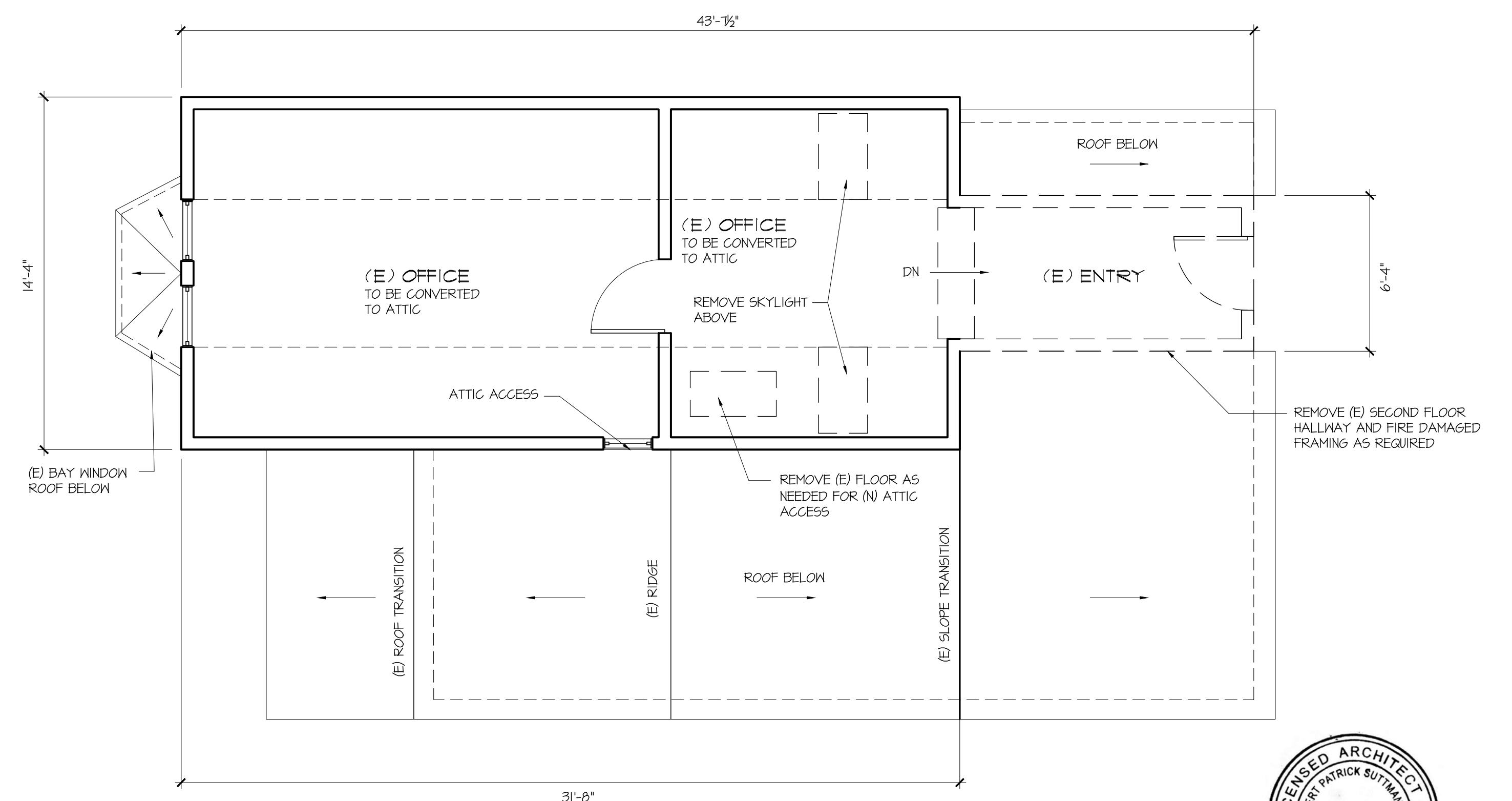
3 - 1/4"=1'-0" SECOND FLOOR DEMOLITION PLAN
