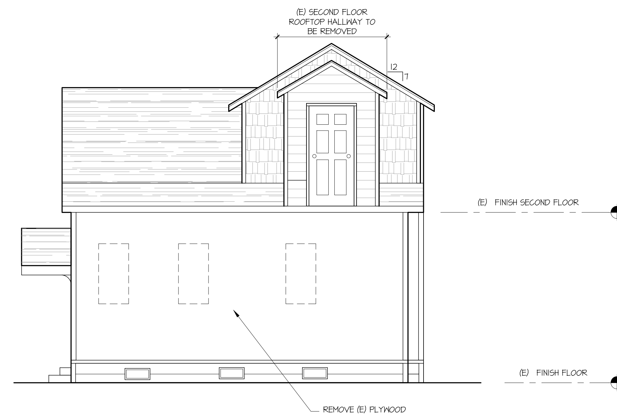
4 EXISTING NORTH ELEVATION 1/4"=1'-0"
