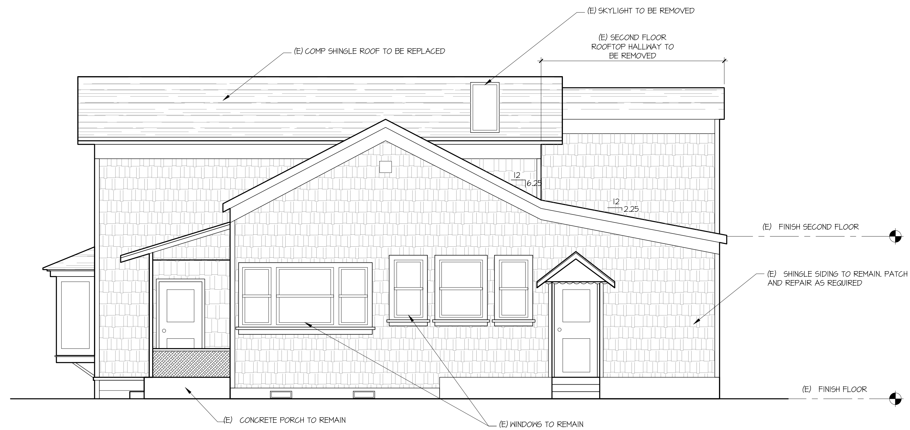
1 EXISTING EAST ELEVATION 1/4"=1'-0"
