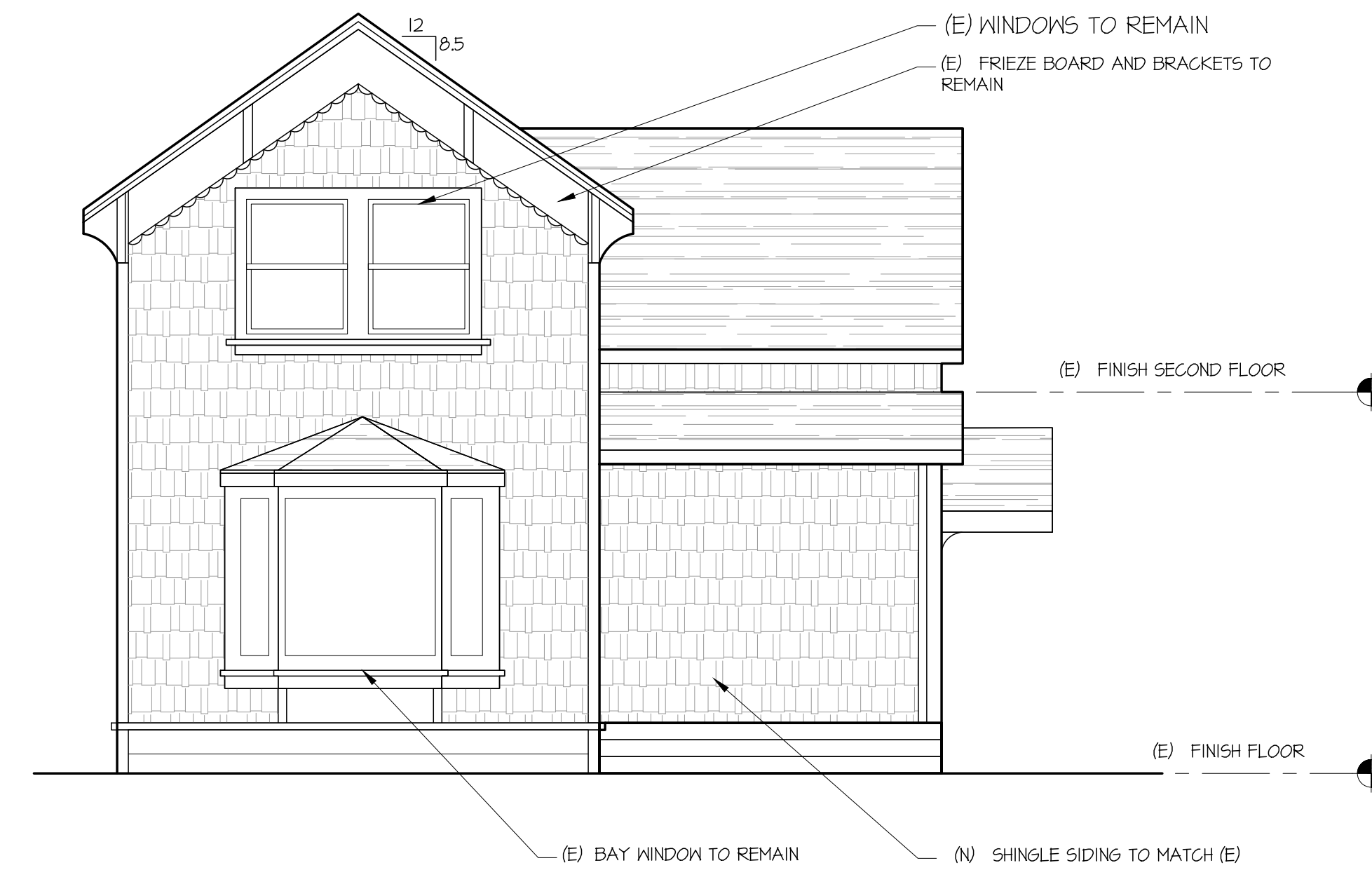
2 PROPOSED SOUTH ELEVATION 1/4"=1'-0"
