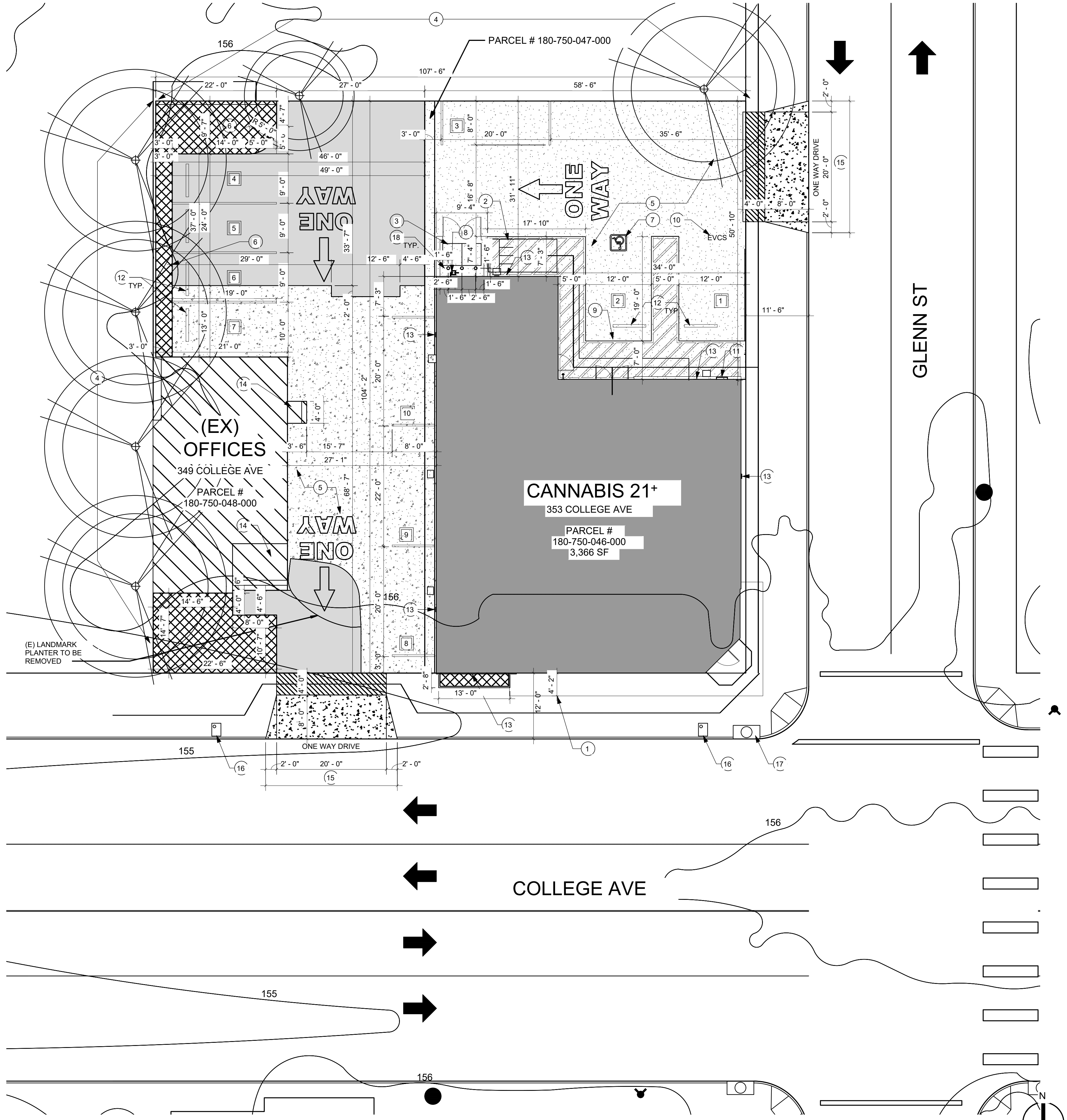
1 PROPOSED SITE PLAN - ENLARGED 1" = 10'-0"
