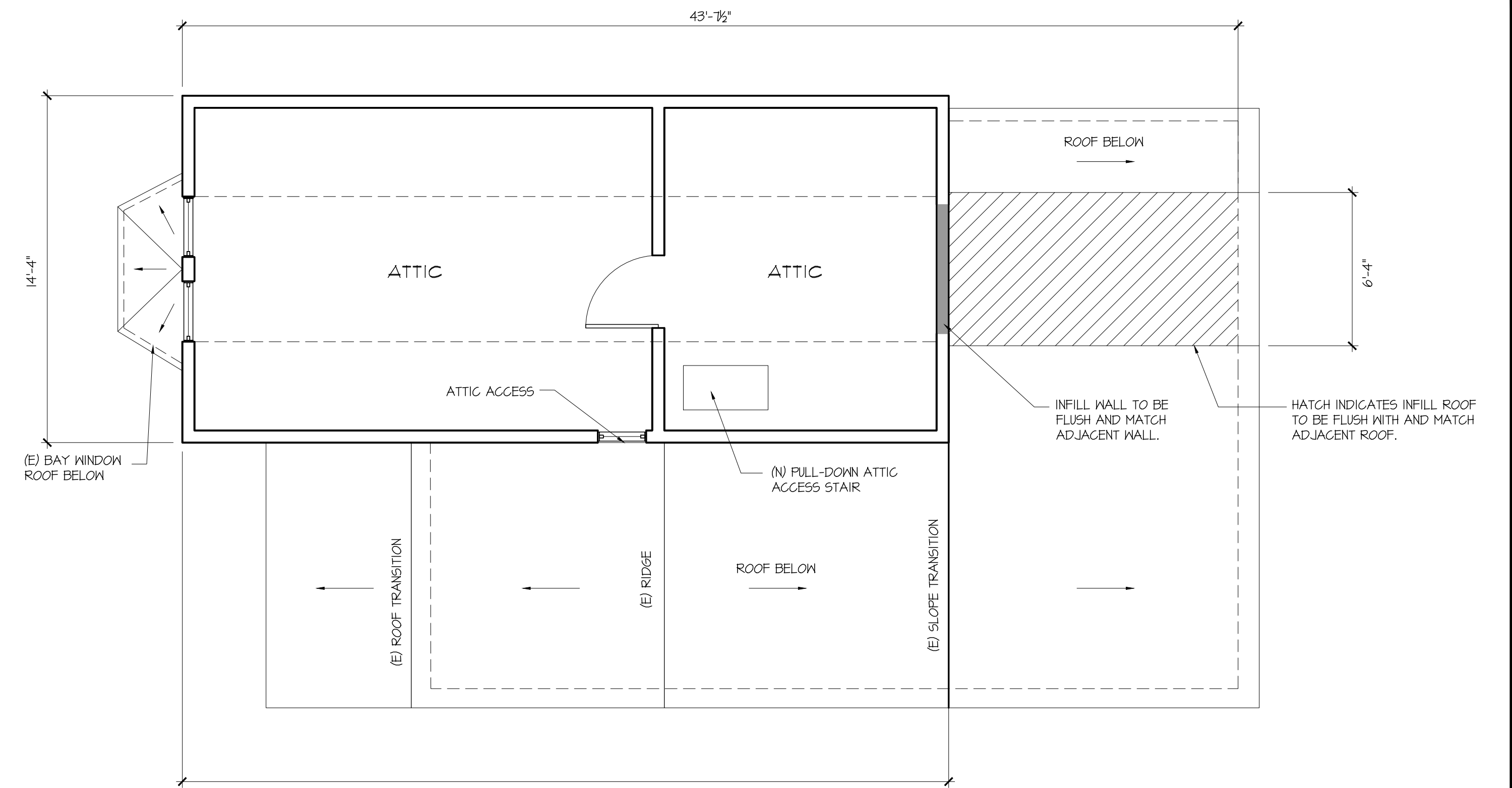
2 - 1/4"=1'-0" PROPOSED SECOND FLOOR PLAN
