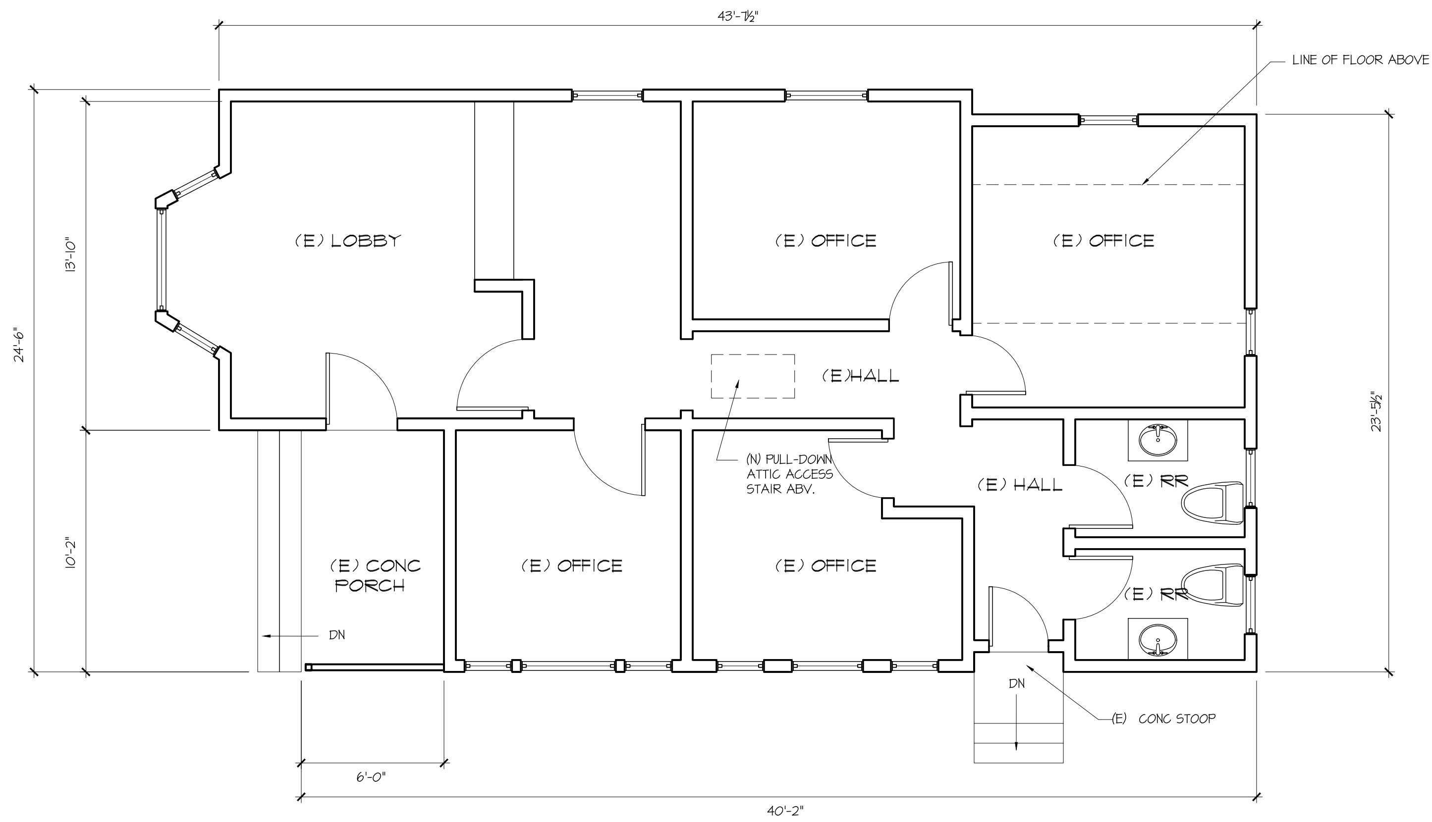
1 - 1/4"=1'-0" PROPOSED FIRST FLOOR PLAN
