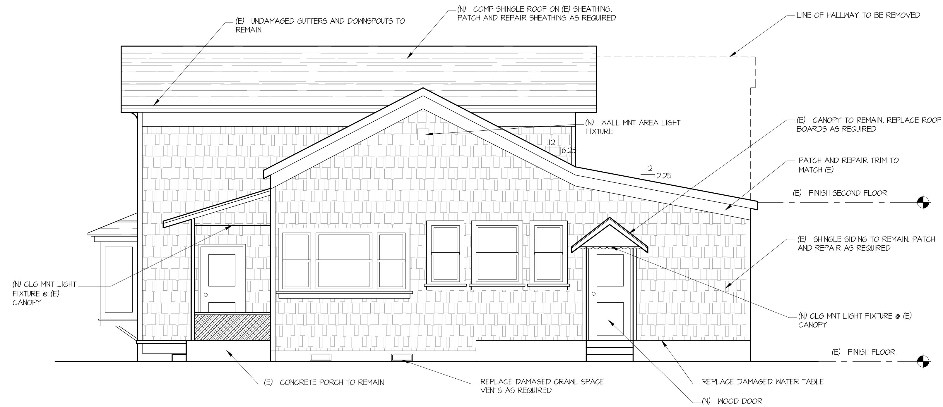
1 PROPOSED EAST ELEVATION 1/4"=1'-0"
