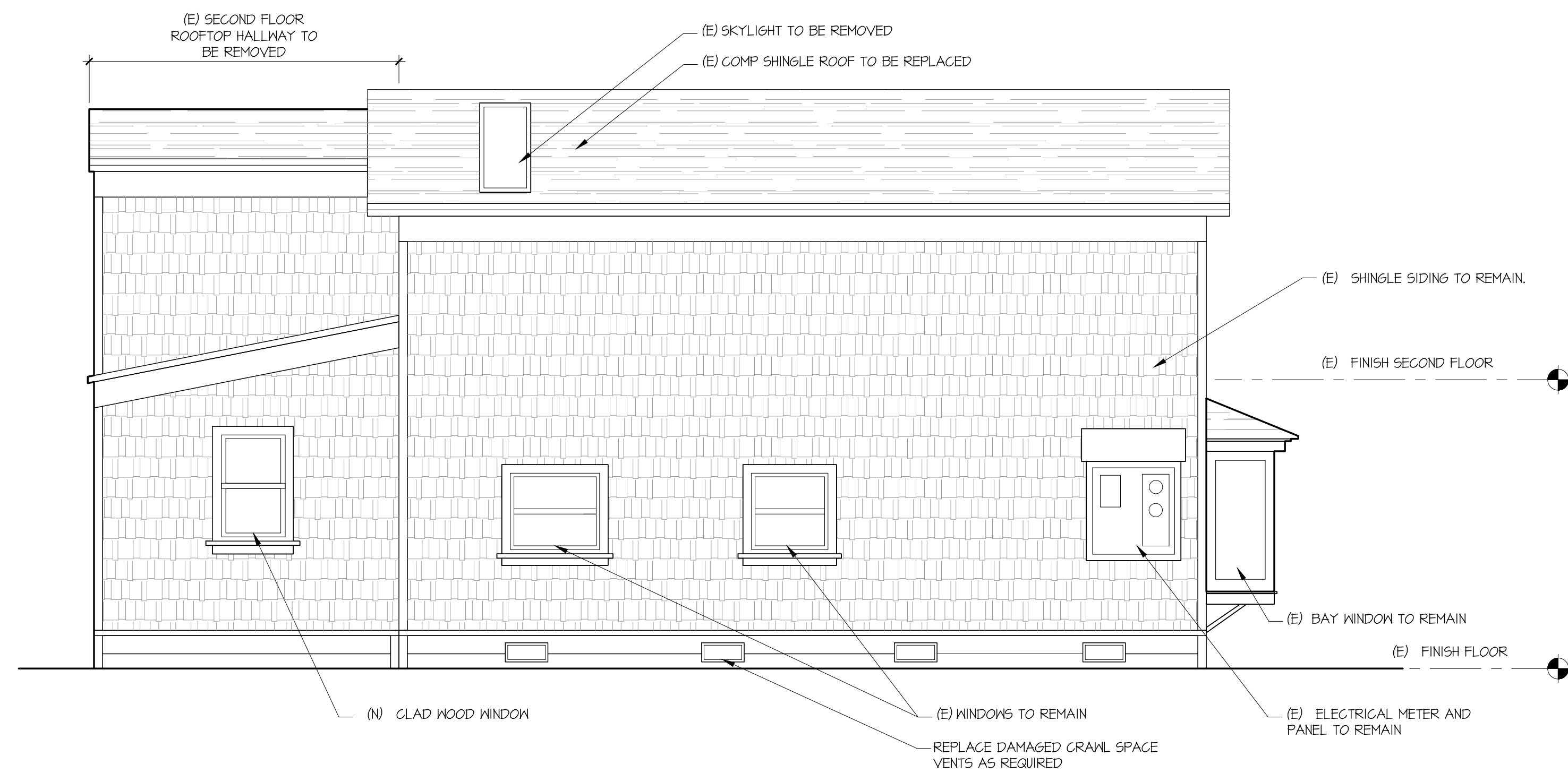
3 EXISTING WEST ELEVATION 1/4"=1'-0"
