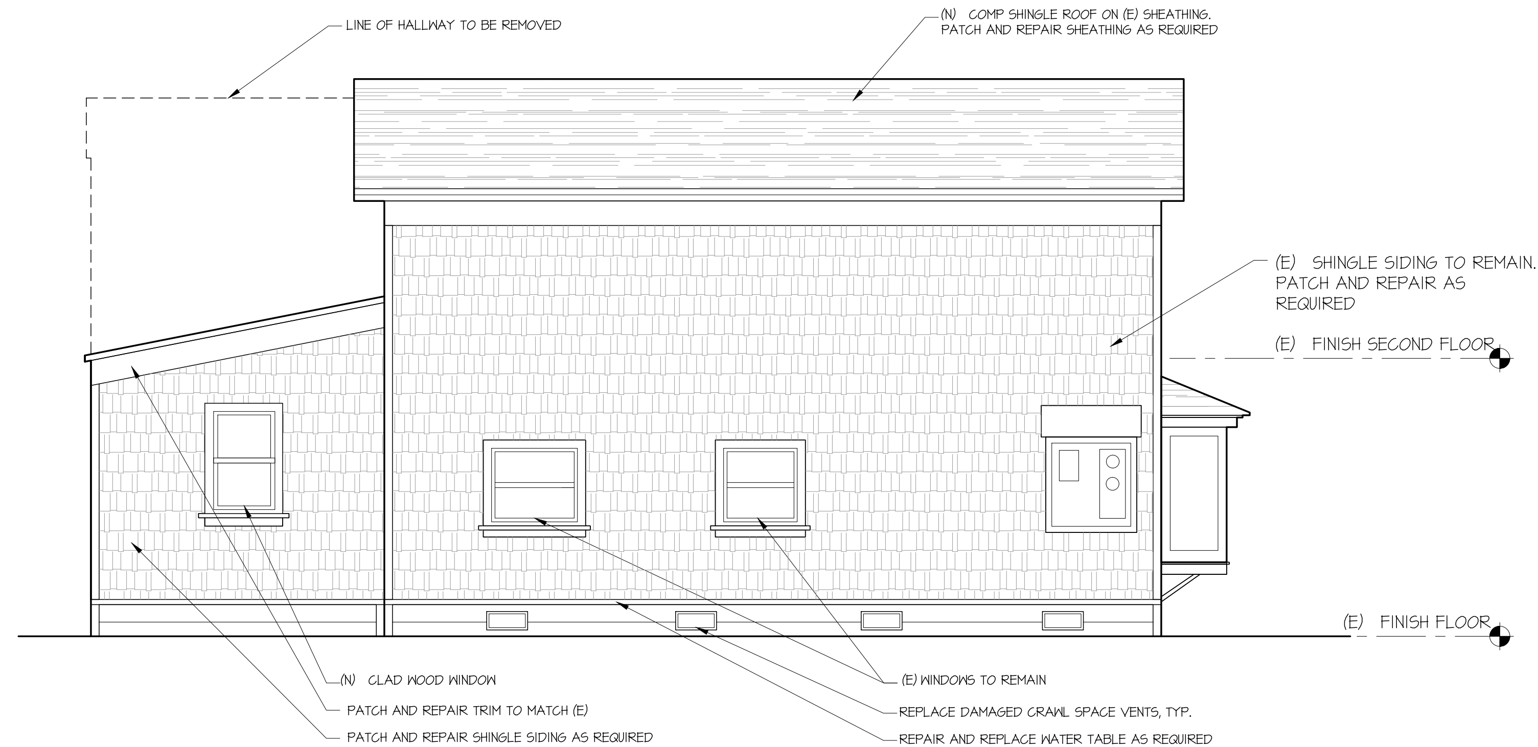
3 PROPOSED WEST ELEVATION 1/4"=1'-0"
