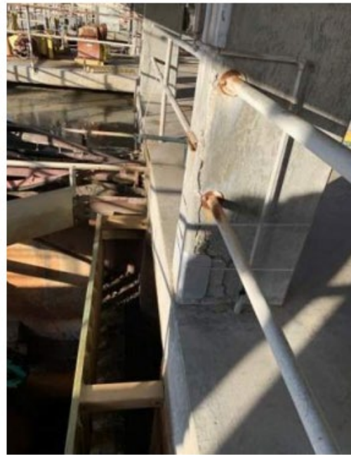
Column Spalling
