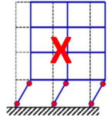
(b) Local failure mechanism
