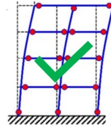
(a) Global failure mechanism
