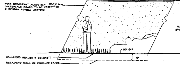
2b SOUND WALL DETAIL - ELEVATION SCALE: NONE
