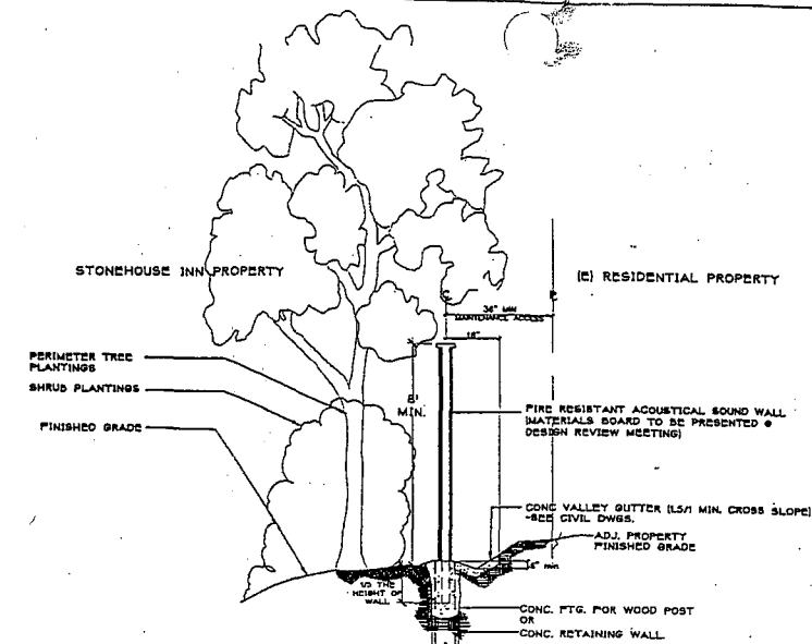
2c SOUND WALL DETAIL SECTION SCALE: NONE
