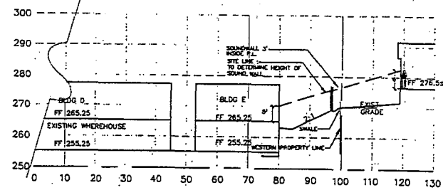
2a SOUND WALL HEIGHT DETAIL AT SECTION B-B SCALE: 1=20
