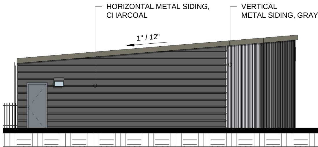
Building C Lot 3 East Elevation
