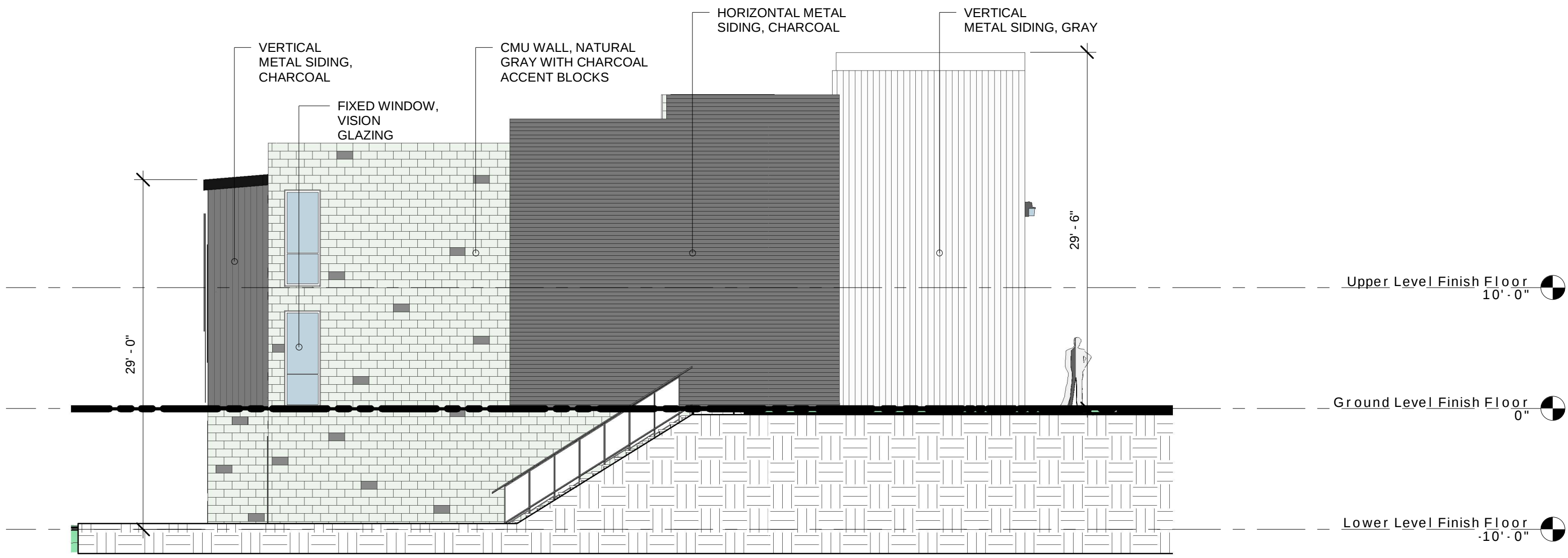
Buiding A Lot 2 East Elevation
