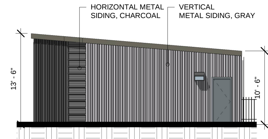
Building B Lot 3 West Elevation
