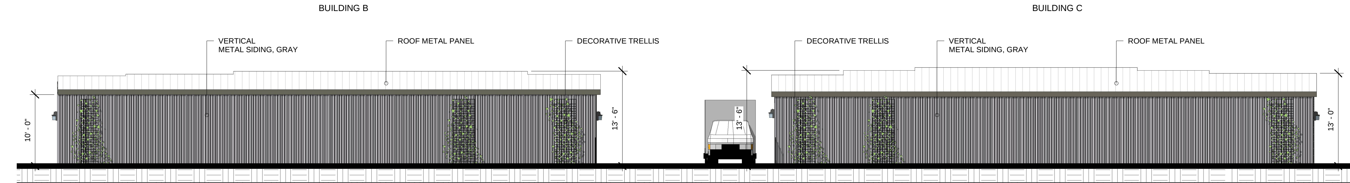
Building B and C Lot 3 South Elevation
