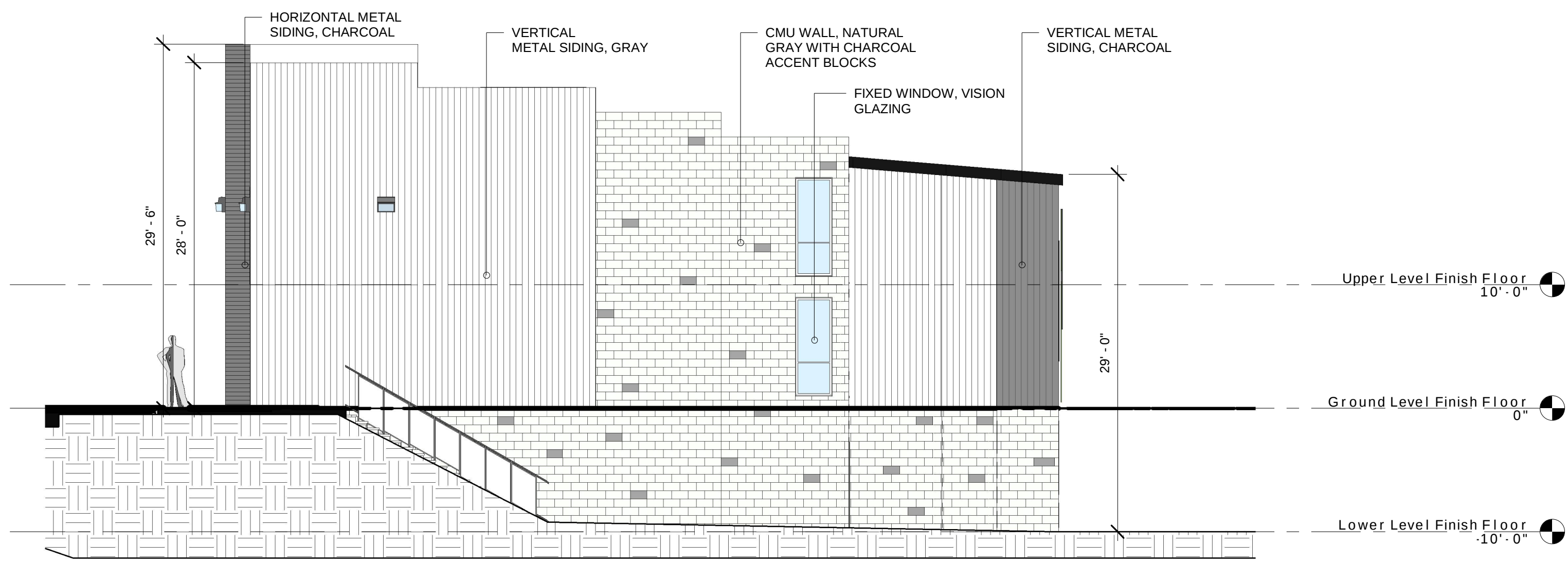
Buiding A Lot 2 West Elevation
