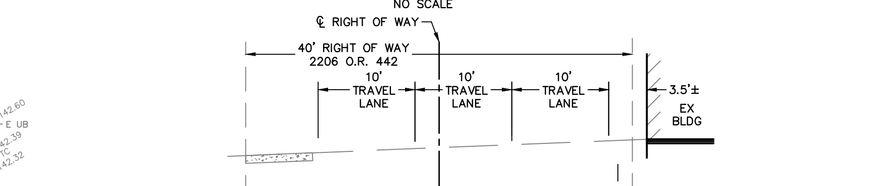
STREET D SOUTH TYPICAL SECTION
