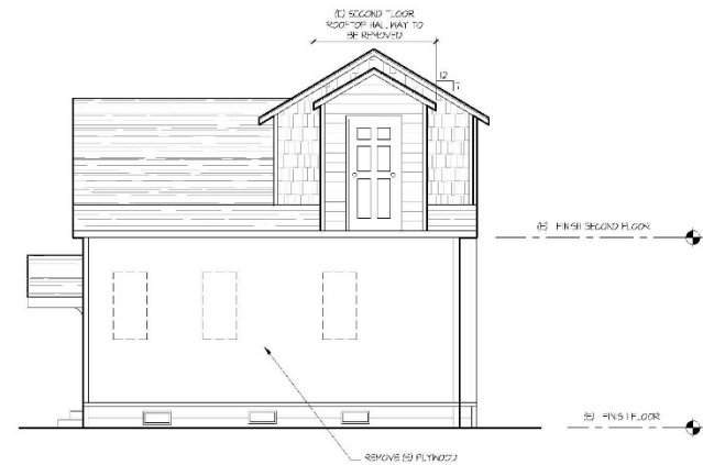
4 EXISTING NORTH ELEVATION
