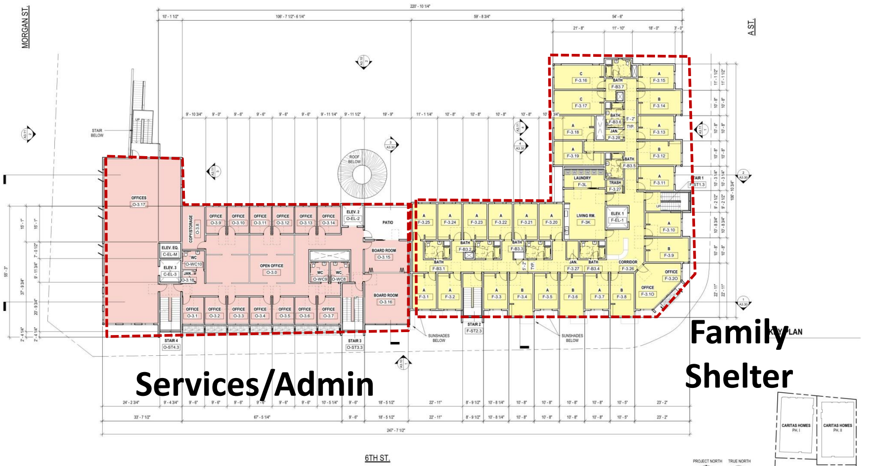
CARITAS CENTER - FLOOR PLAN - LEVEL 3 1" = 10'-0"
