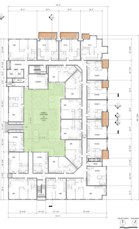
CARTAS HOMES - FLOOR PLAN - LEVEL 2
