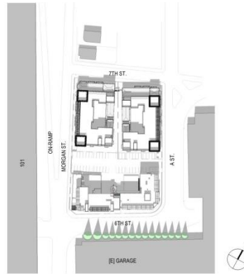
SHADOW STUDY - SEPTEMBER 21ST, 12PM 1" = 100'-0" 5
