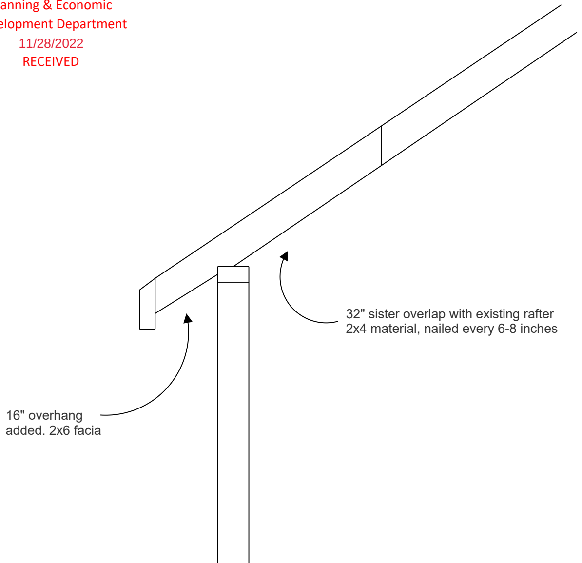
1209 12th Street, Sant Rosa CA Rafter Extension Detail
