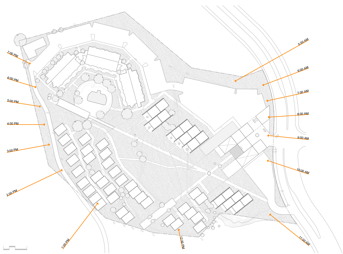
Summer Solstice Sun-path
