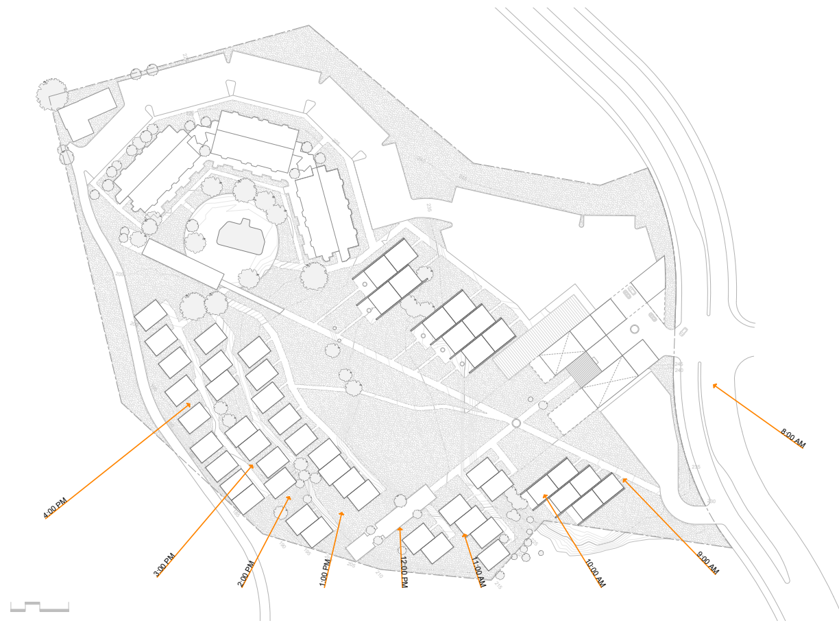
Winter Solstice Sun-path
