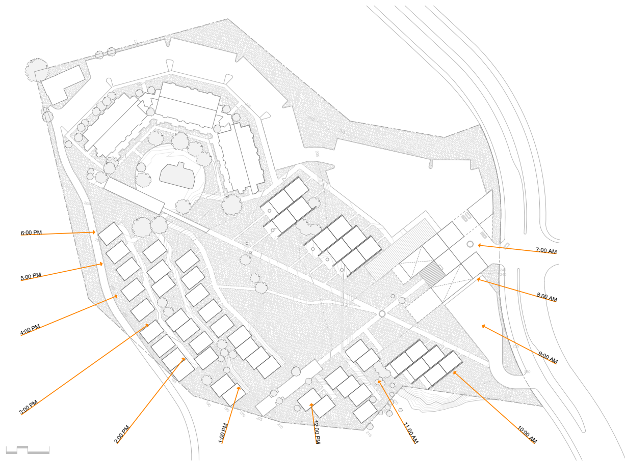
Spring/Fall Equinox Sun-path
