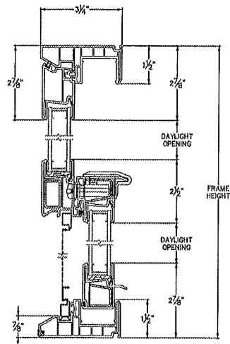
HEAD & SILL
