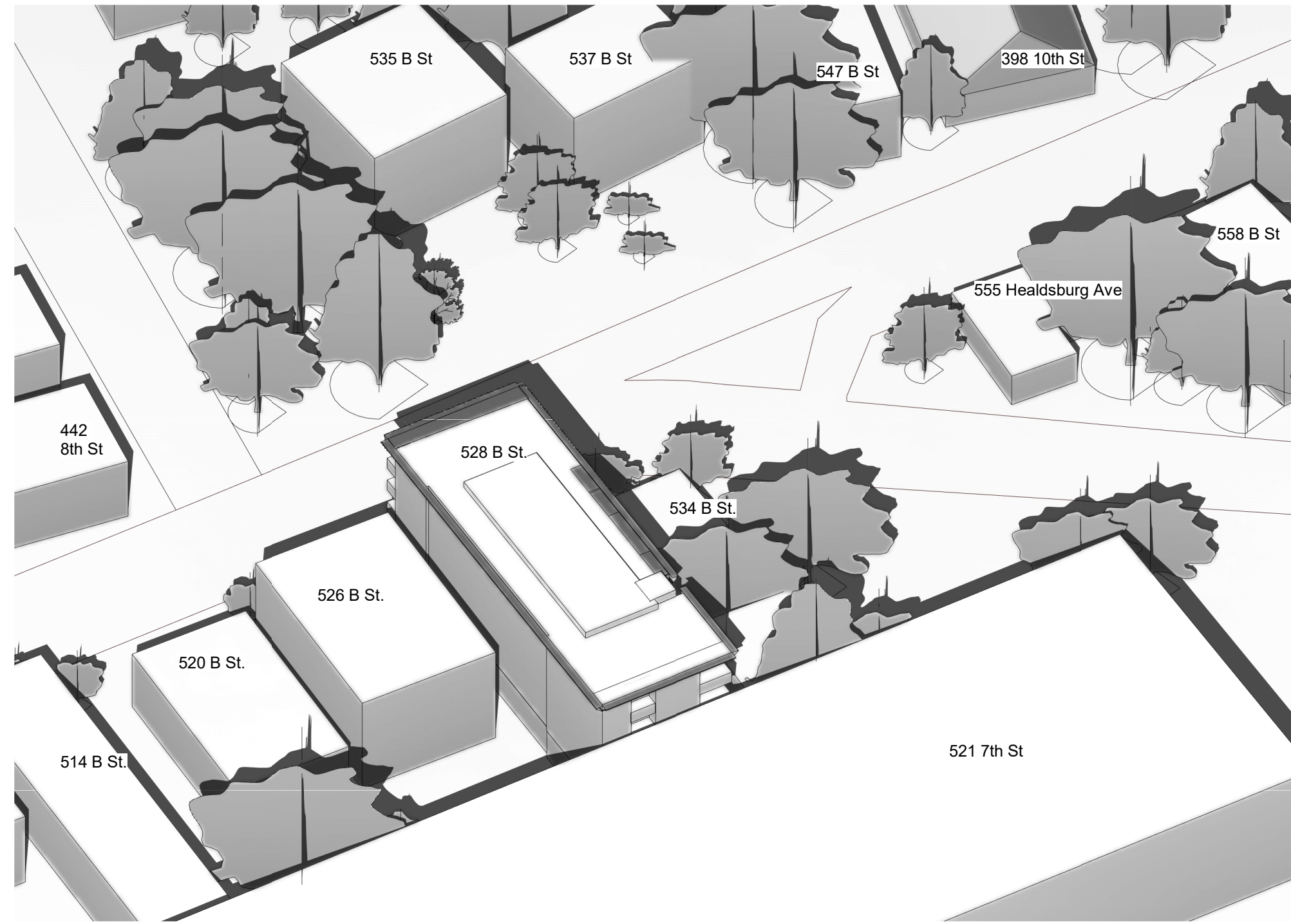
3 8AM - 6/20 - EAST VIEW
