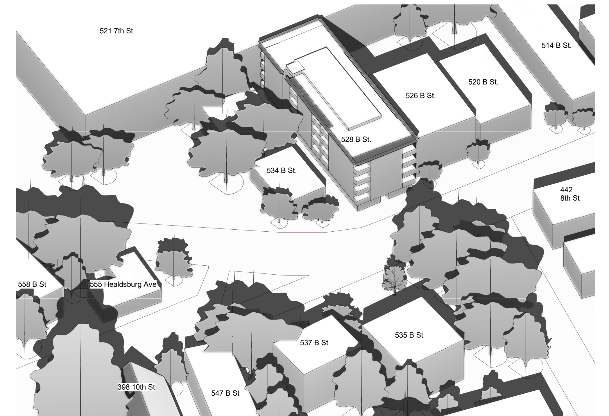
5 4PM - 6/20 - WEST VIEW
