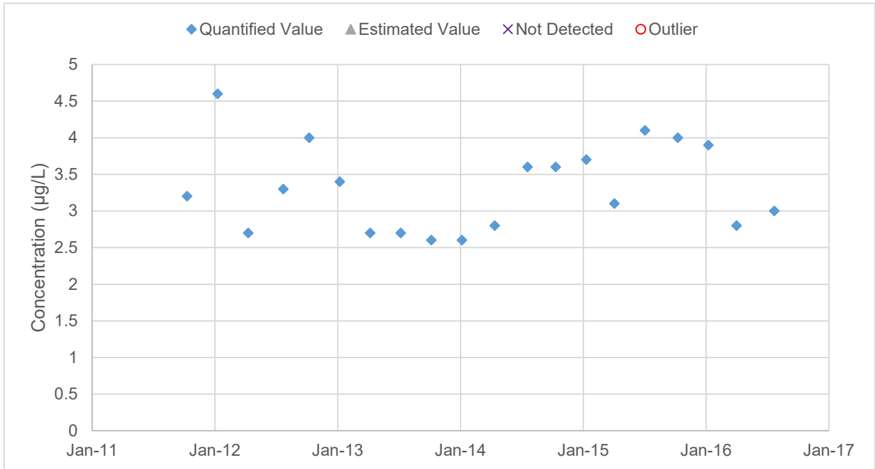
Figure B-9: Chromium Concentration in Facility Influent
