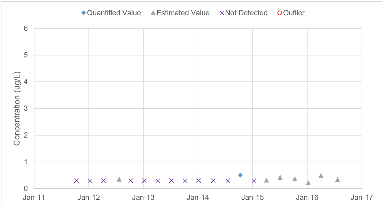
Figure B-16: Lead Concentration in Facility Effluent
