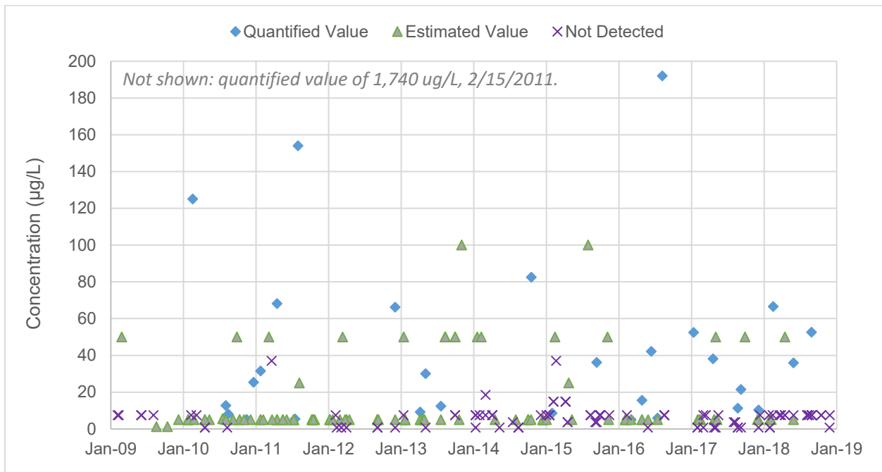
Figure B-49: Bis (2-ethylhexyl) phthalate Concentration in Industrial Wastewater
