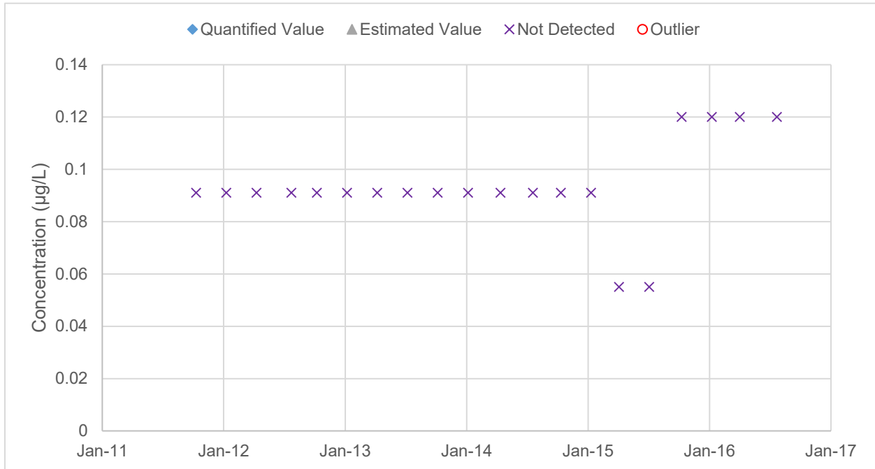
Figure B-5: Beryllium Concentration in Facility Influent
