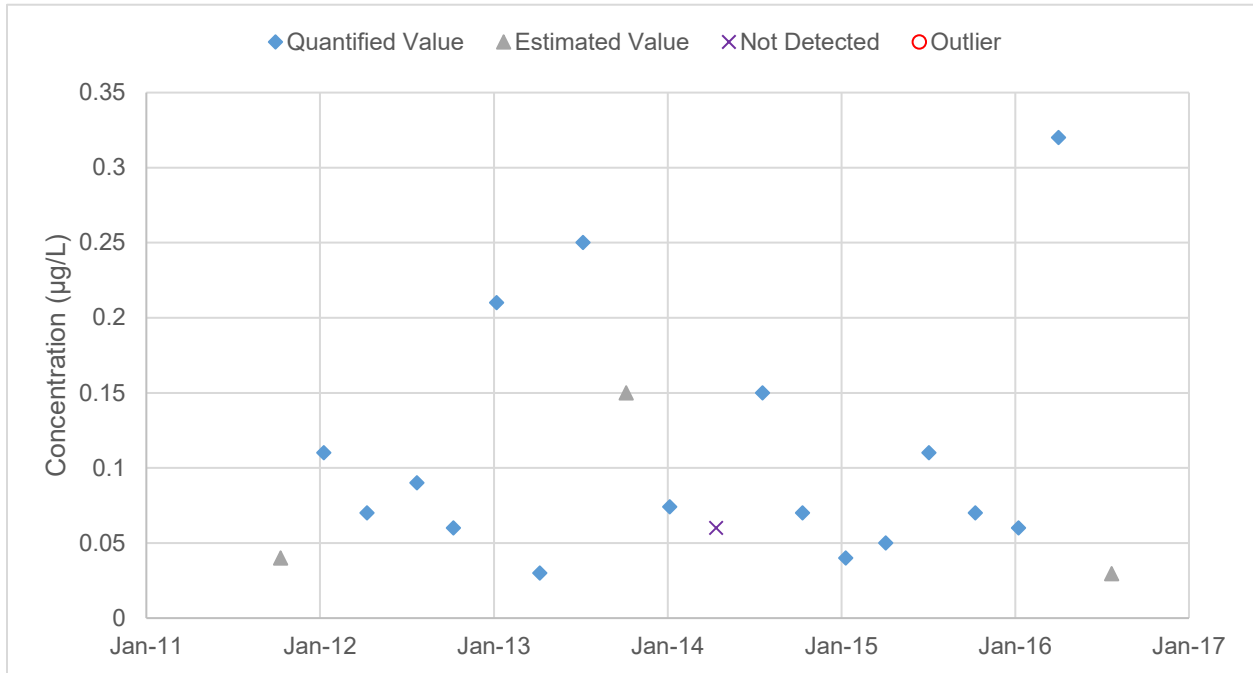
Figure B-17: Mercury Concentration in Facility Influent
