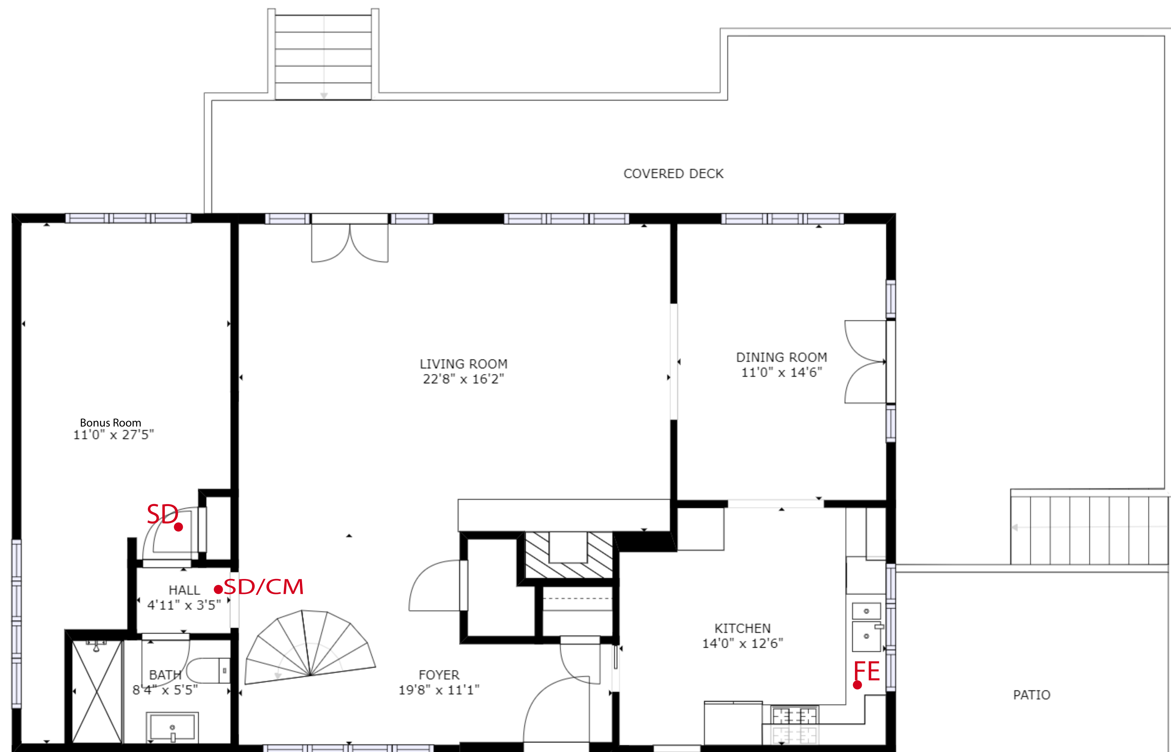
FLOOR 1
