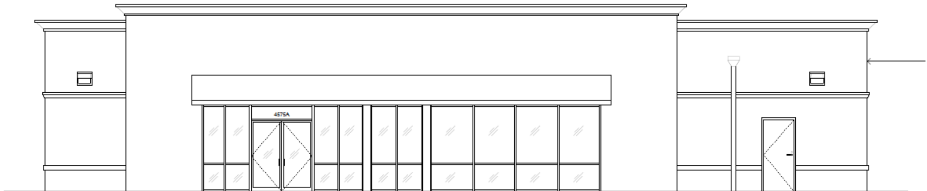
NORTHWEST EXTERIOR ELEVATION
