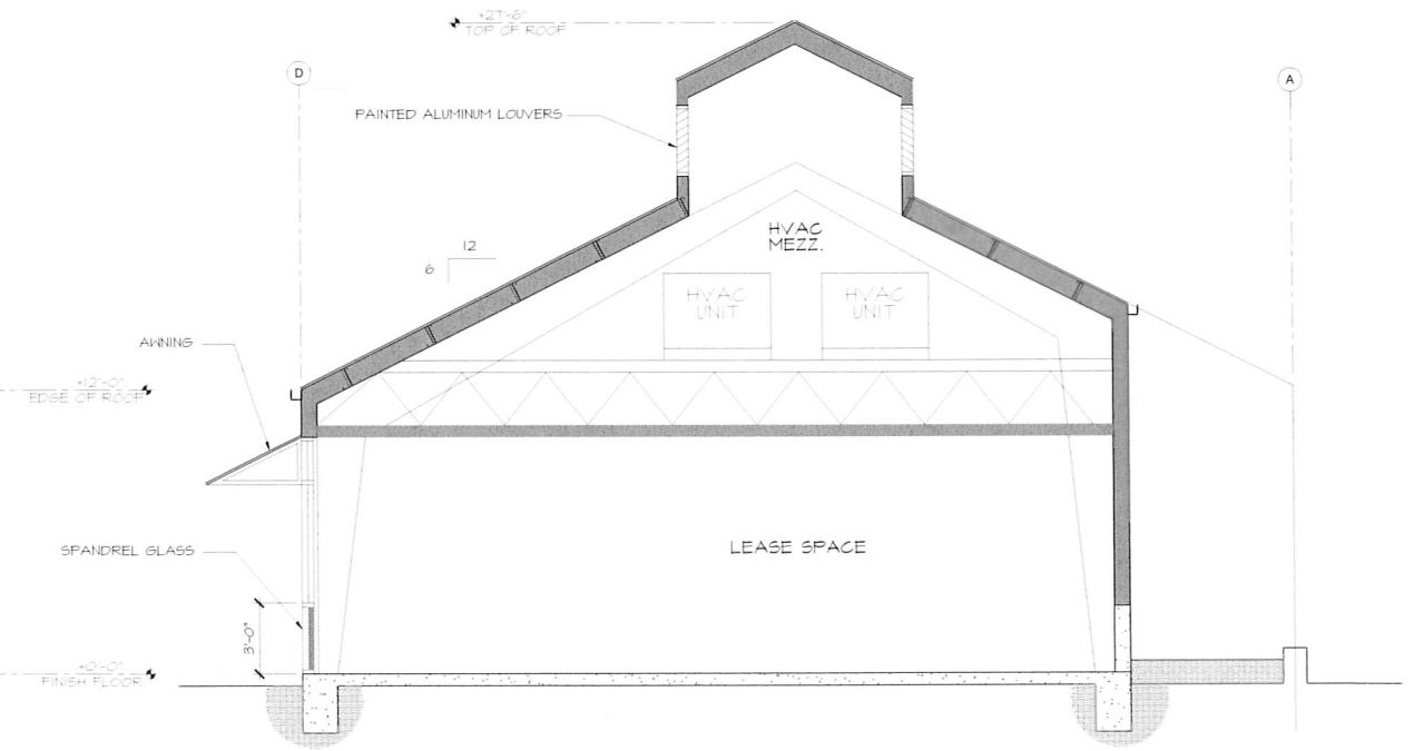
4 BUILDING 'A' SECTION 1/4" = 1'-0"
