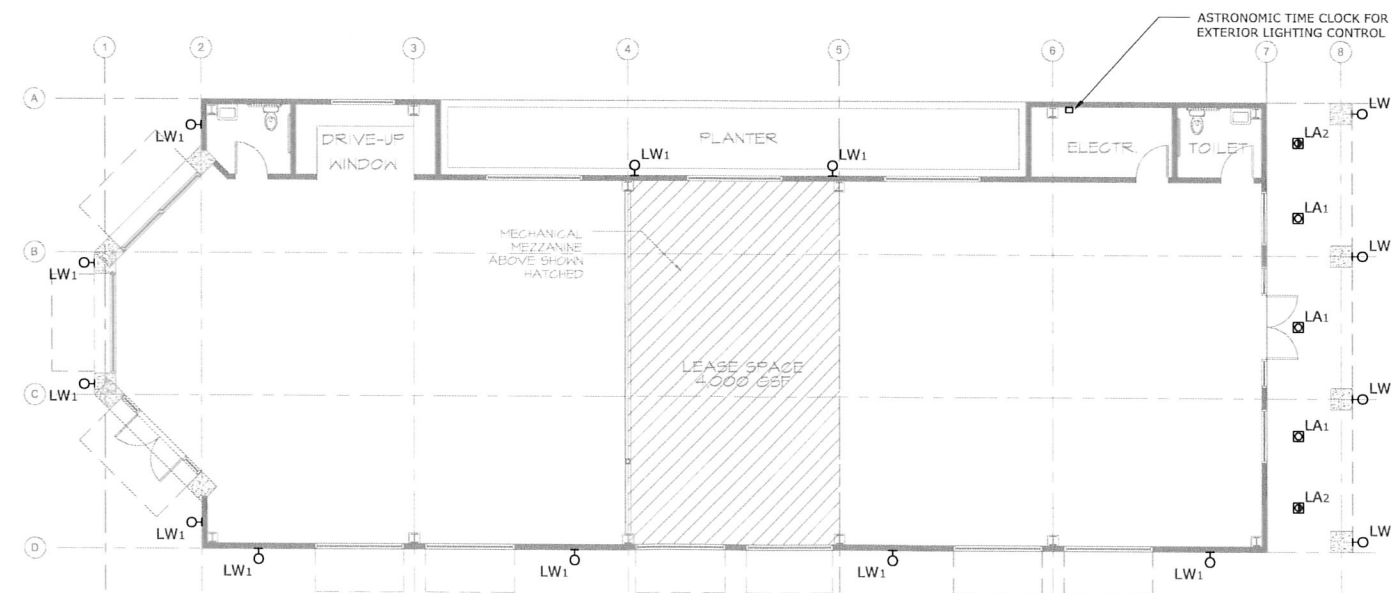
② BUILDING 'A' FLOOR PLAN 1/8" = 1'-0"
