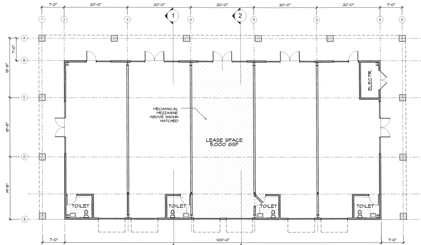
① BUILDING 'B' FLOOR PLAN 1/8" = 1'-0"
