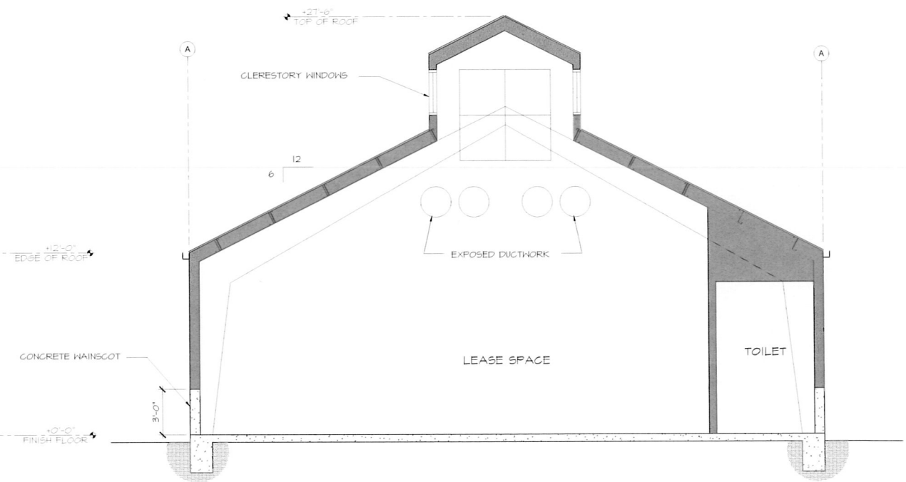
3 BUILDING 'A' SECTION 1/4" = 1'-0"
