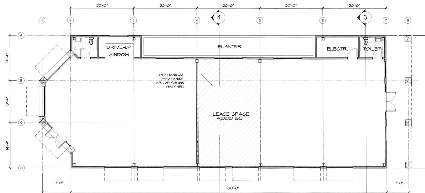
② BUILDING 'A' FLOOR PLAN 1/8" = 1'-0"
