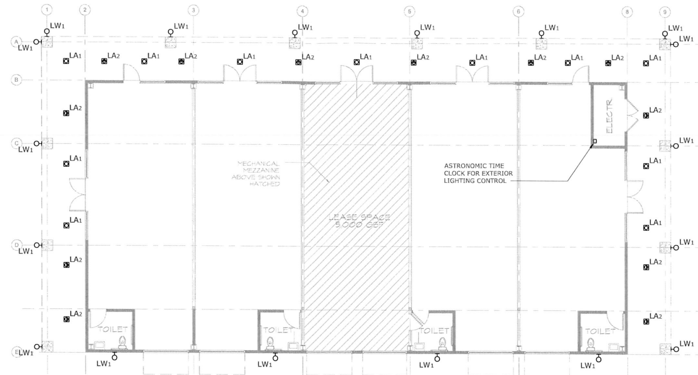
① BUILDING 'B' FLOOR PLAN 1/8" = 1'-0"
