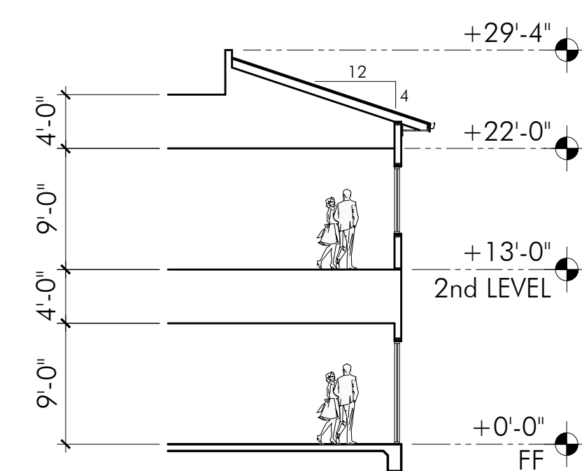
BLDG SECTION A-A
