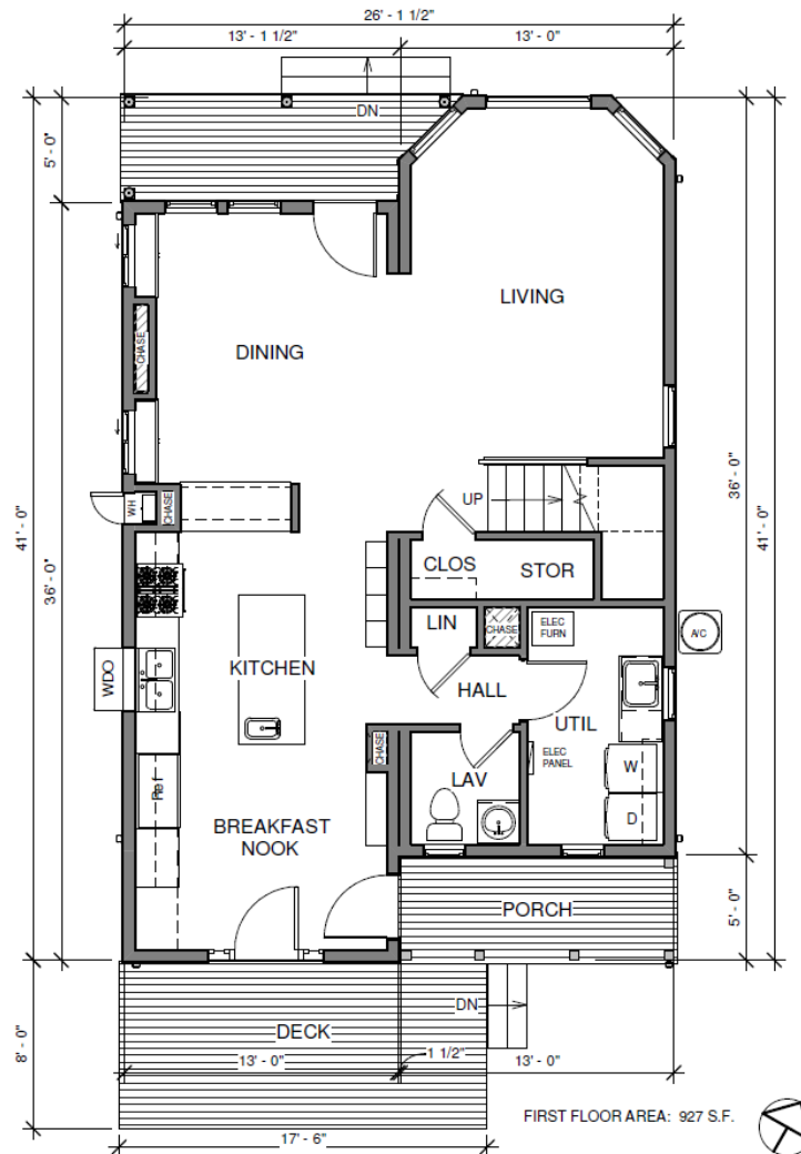
① 1ST FLOOR PRESENTATION 3/16" = 1'-0"
