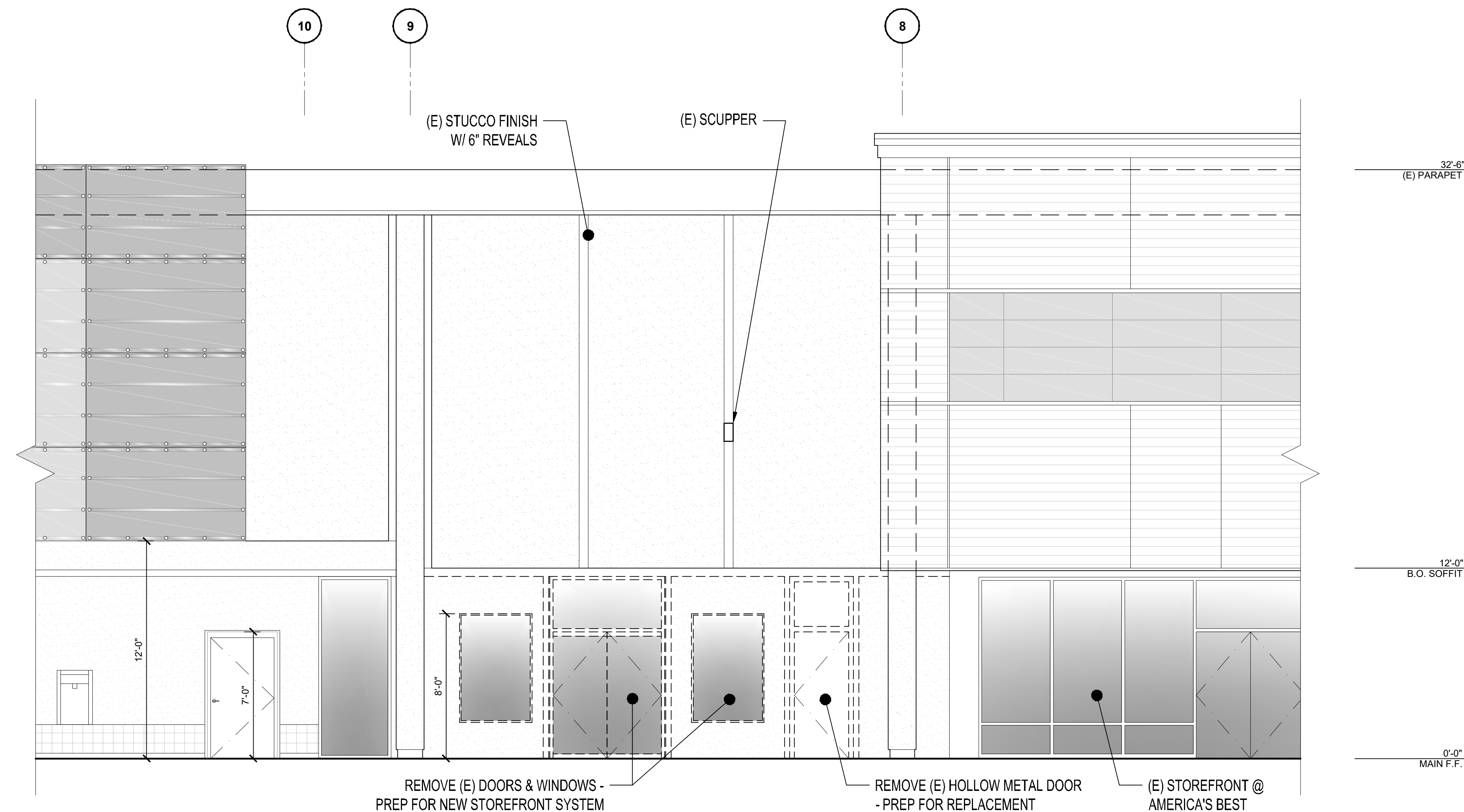
2 EXISTING NORTH ELEVATION A2.0 1/4" = 1'-0"
