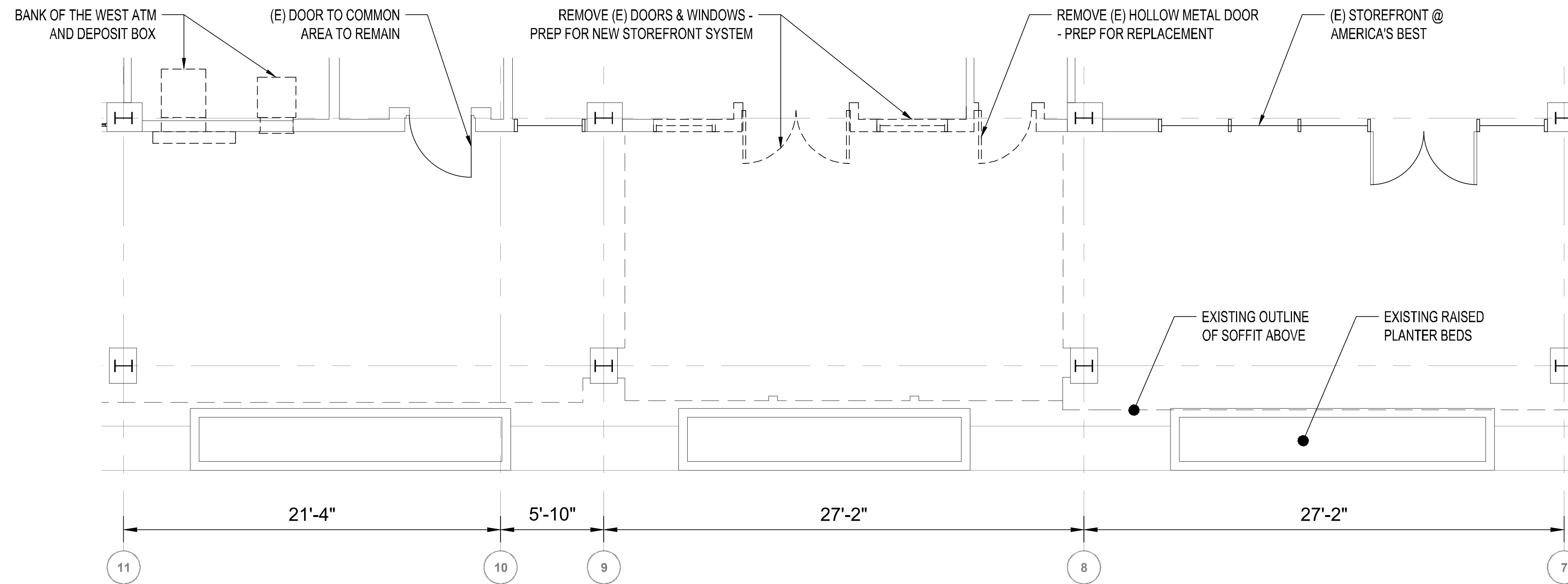
1 EXISTING FLOOR PLAN A2.0 1/4" = 1'-0"
