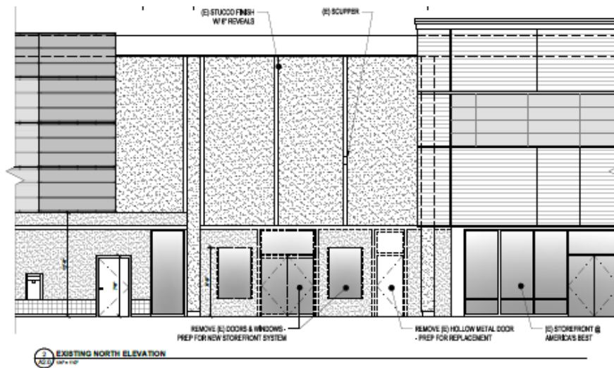
Existing Elevation
