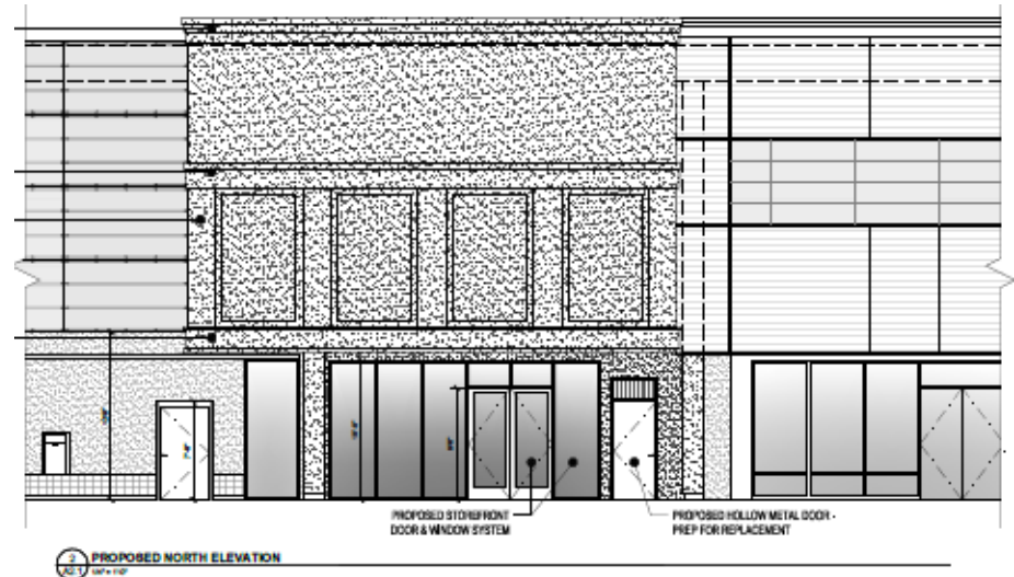
Proposed Elevation
