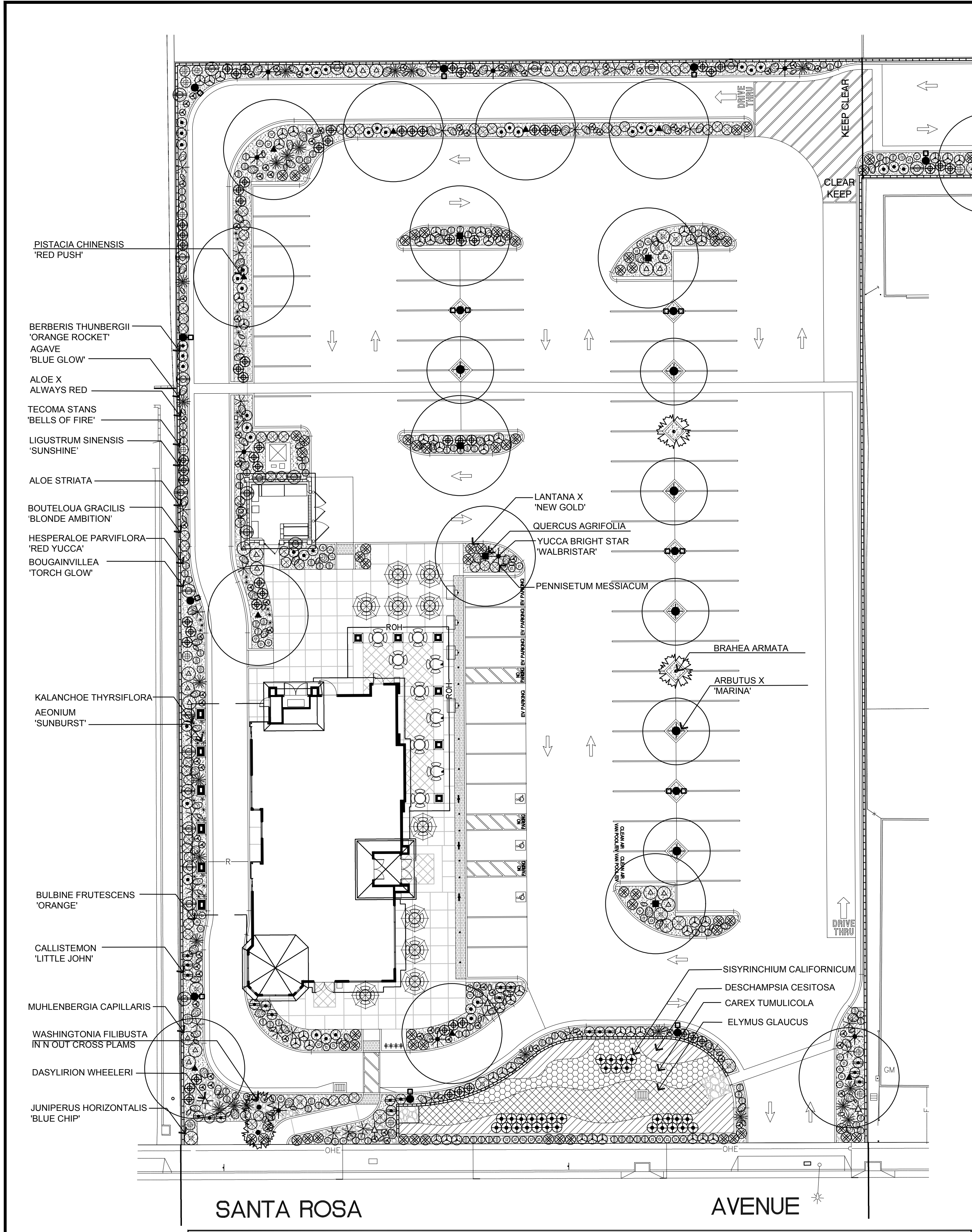
PLAN VIEW
