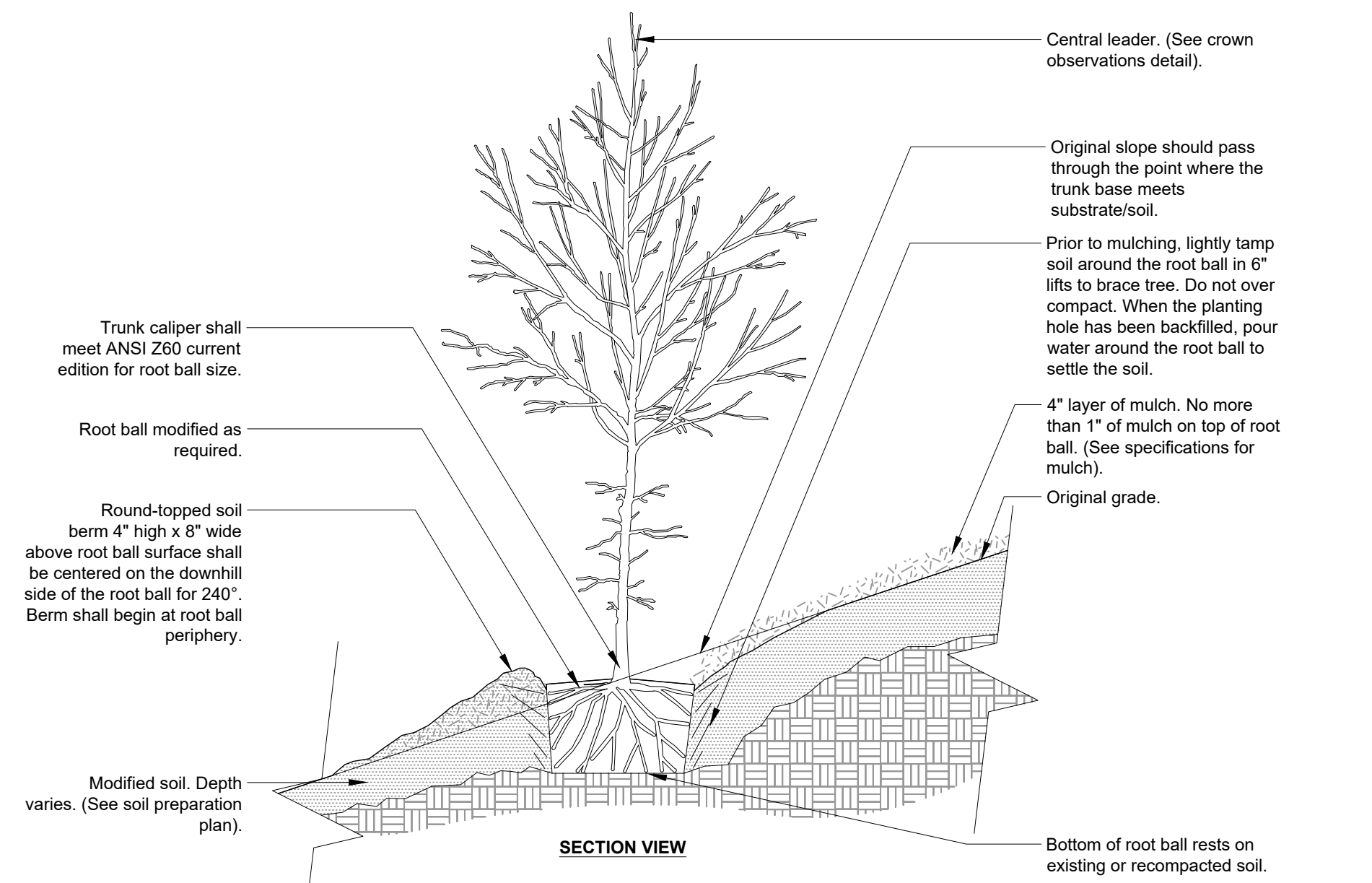
TREE ON SLOPE 5% (20:1) TO 50% (2:1) (EXISTING SOIL MODIFIED)
