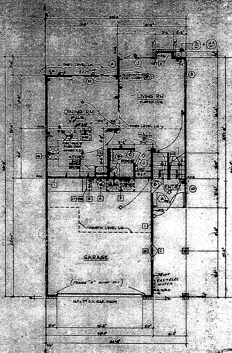
FIRST & SECOND LEVEL FLOOR PLAN
