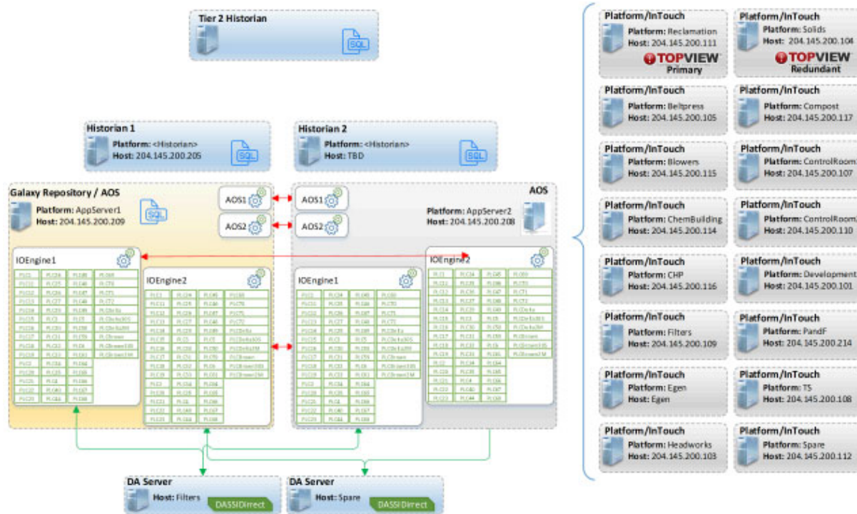
Figure 1 - Existing System Architecture
