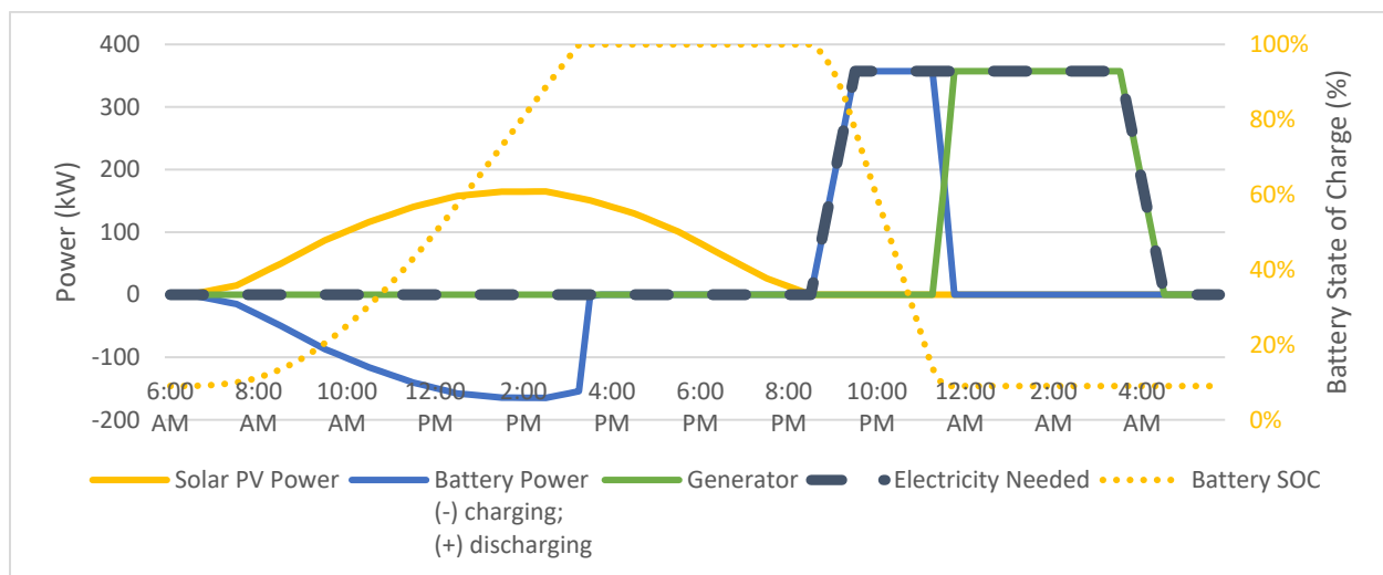
Figure 10. PV, BESS, and PG&E Grid load profile during a 24-hour outage operation at Utilities Field Operations.
