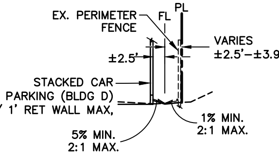
SECTION D-D 1" = 20' HORZ. 1" = 10' VERT.
