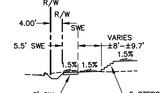
SECTION G-G 1" = 20' HORZ. 1" = 10' VERT.
