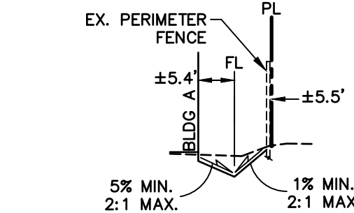
SECTION C-C 1" = 20' HORZ. 1" = 10' VERT.
