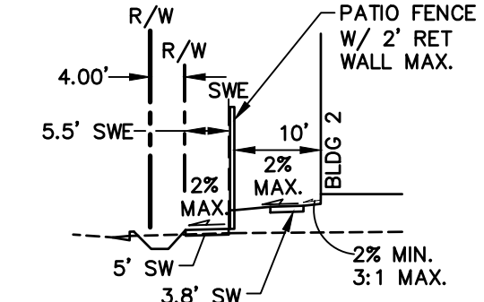
SECTION F-F 1" = 20' HORZ. 1" = 10' VERT.
