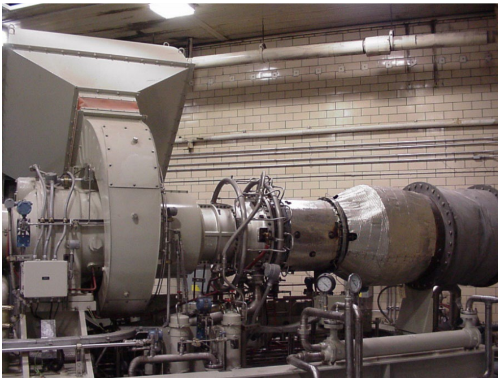
Figure 3-2. Solar Mercury 50 gas turbine at the Village Creek WWTP, Fort Worth, TX
