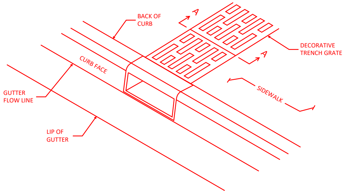
ISOMETRIC VIEW
