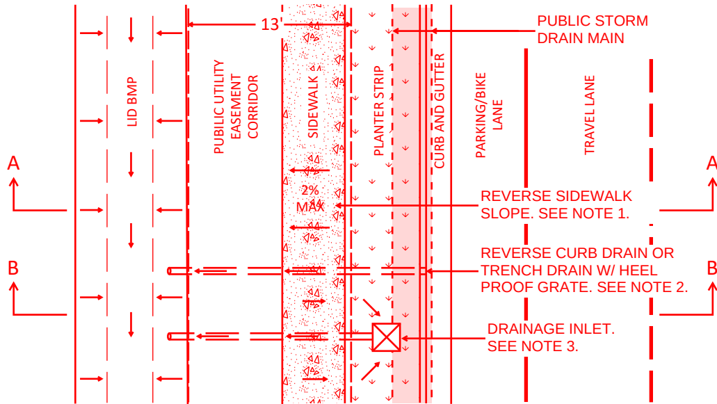
PLAN VIEW
