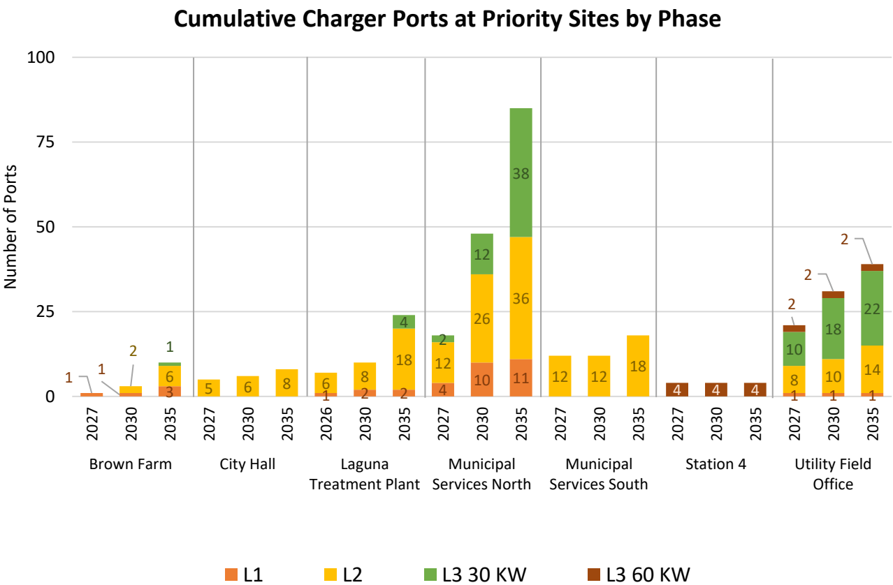
Figure 1. Cumulative charger ports per phase at each priority site
