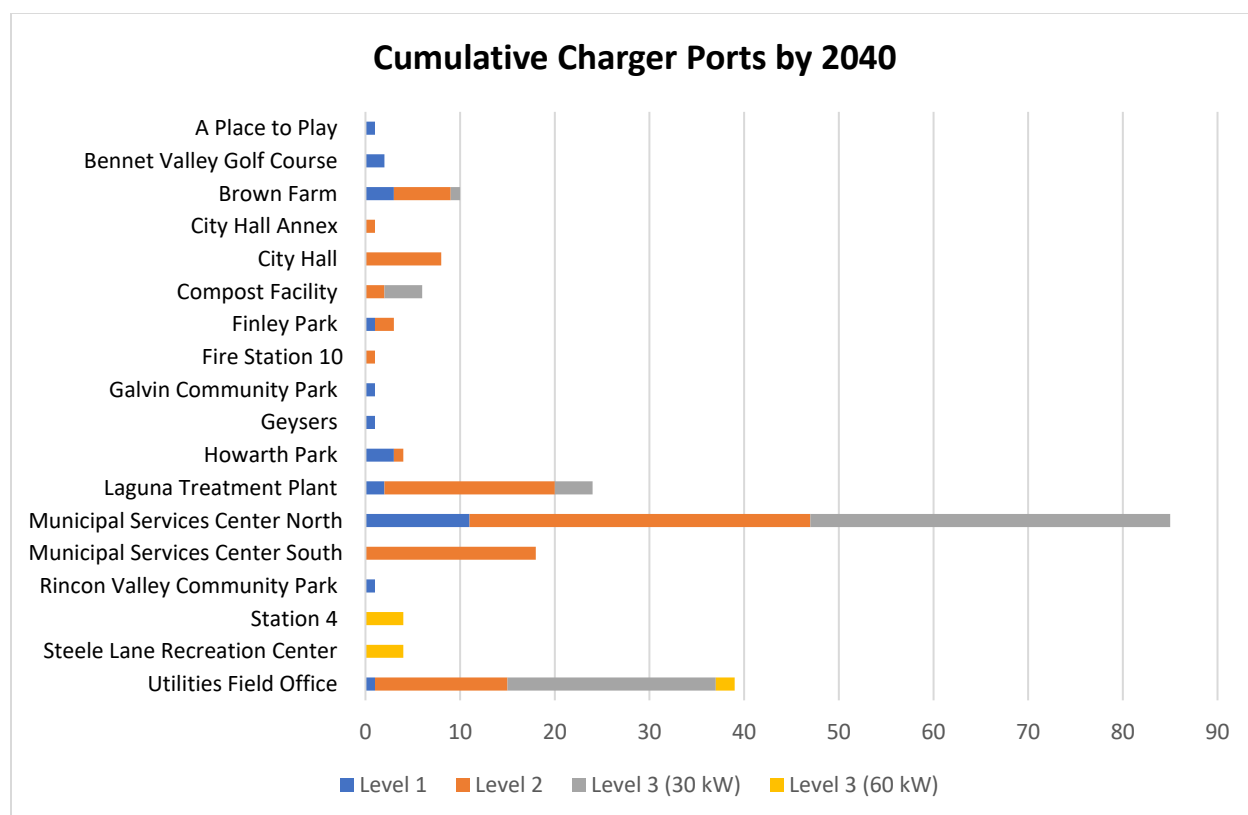
Figure 11. Cumulative quantity of EV charger ports needed for a fully electrified fleet by site.
