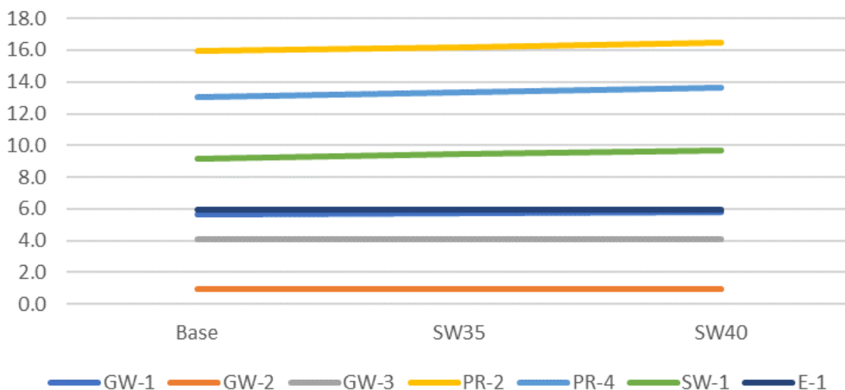
Figure 3-17: Supply Option Cost Performance with Varying Sonoma Water Cutbacks ($M/yr)
