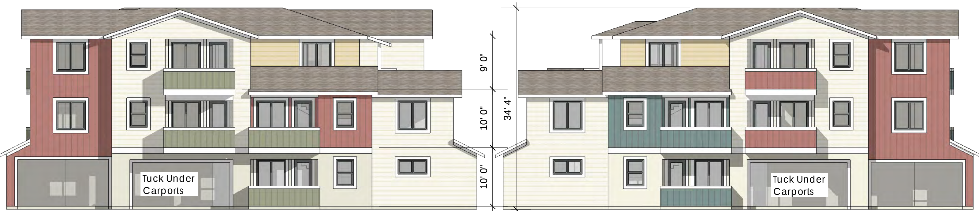
Building 2/ South Elevation
