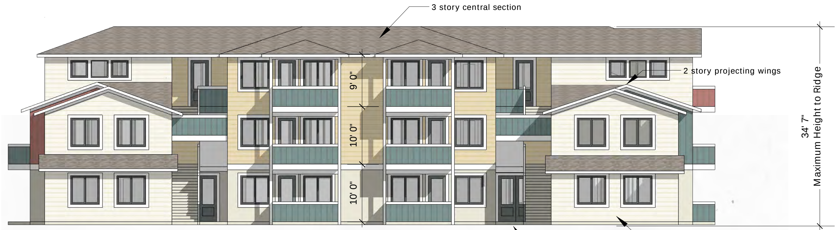
West (Burbank Avenue) Elevation
