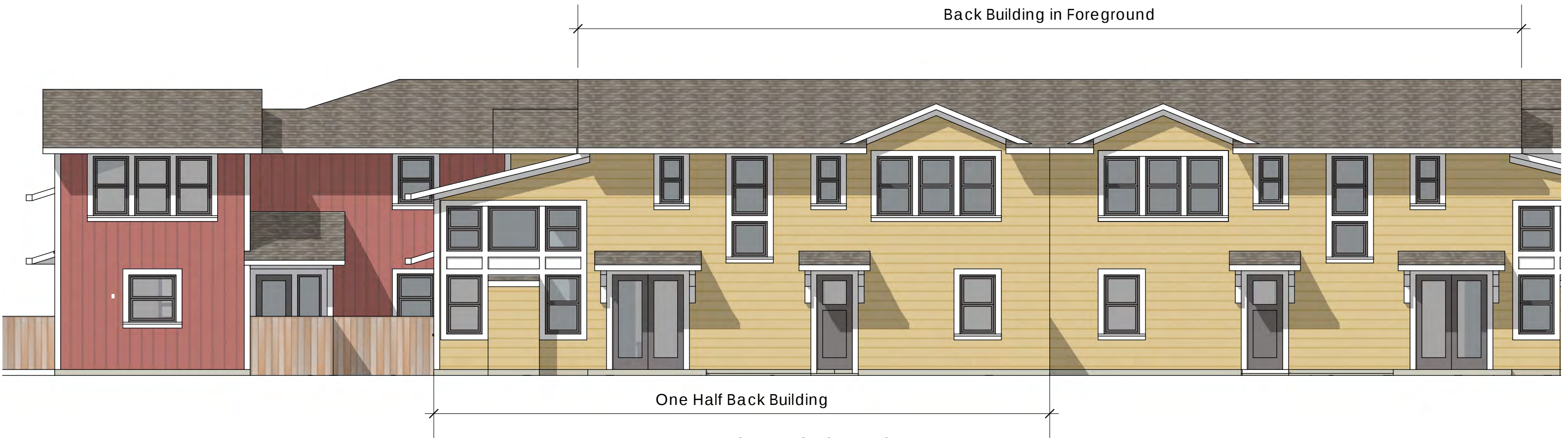
Back Yard Elevation
