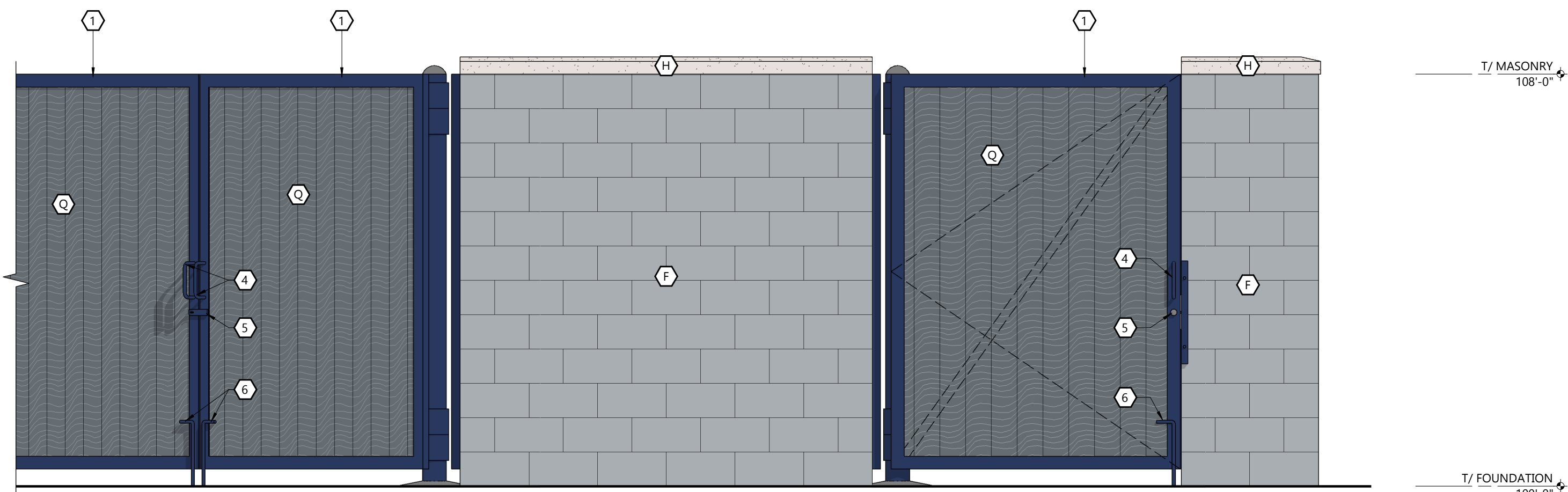
ELEVATION - FRONT
