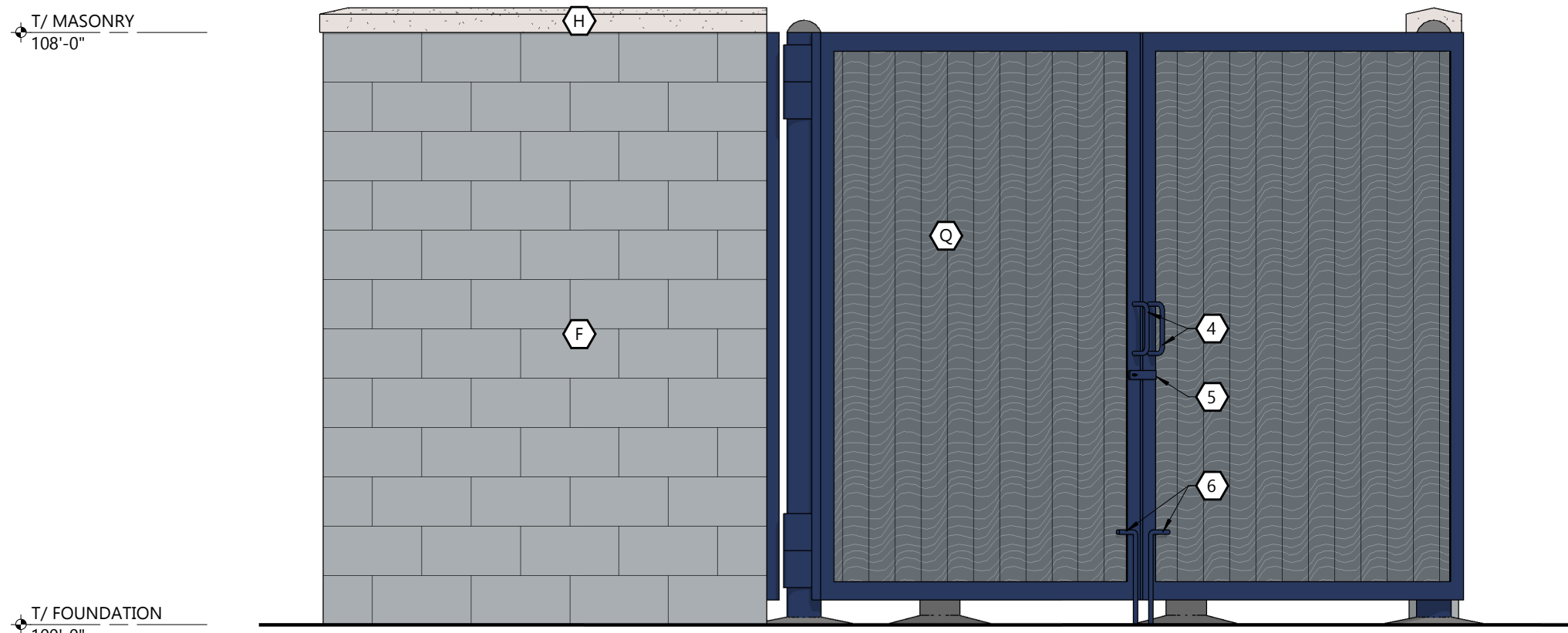
ELEVATION - LEFT
