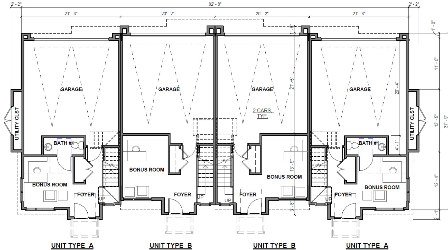
1 1ST FLOOR - 4-PLEX 1/8" = 1'-0"
