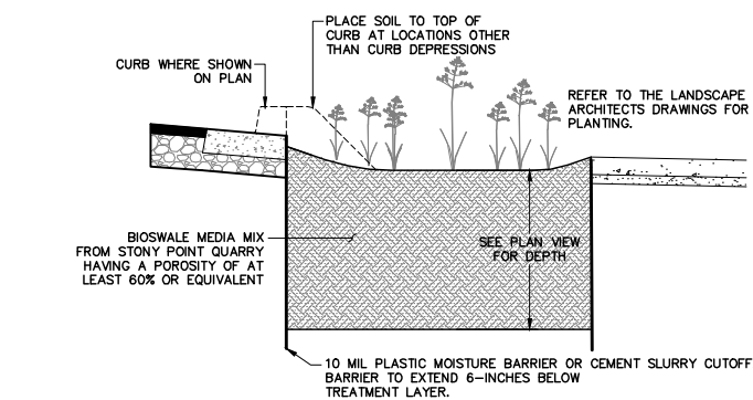
1 BIORETENTION AREA NO SCALE
