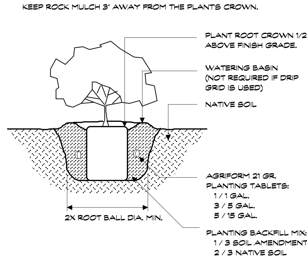
1 Shrub Planting Section 3/4" = 1' 0"
