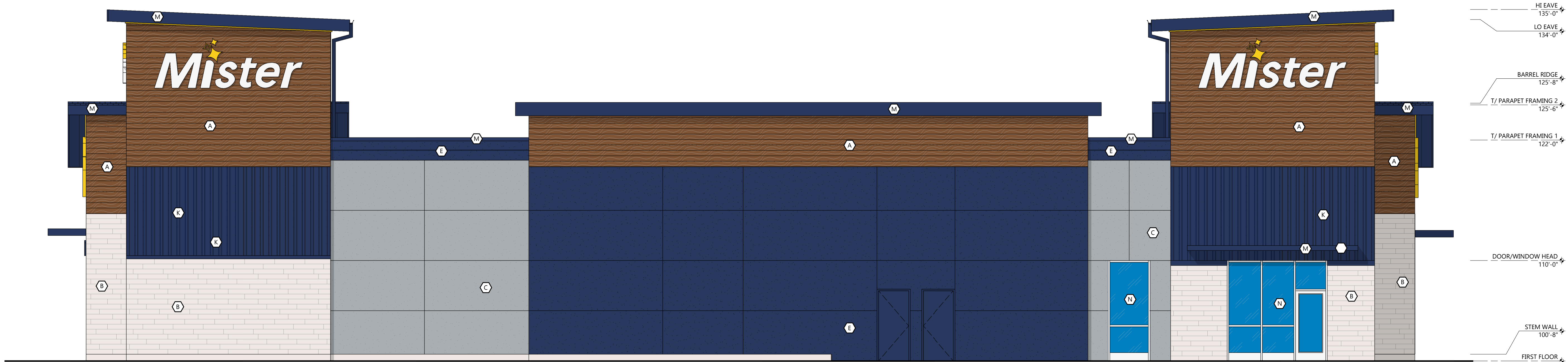
OFFICE ELEVATION (SOUTH) SCALE: 3/16" = 1'-0"
