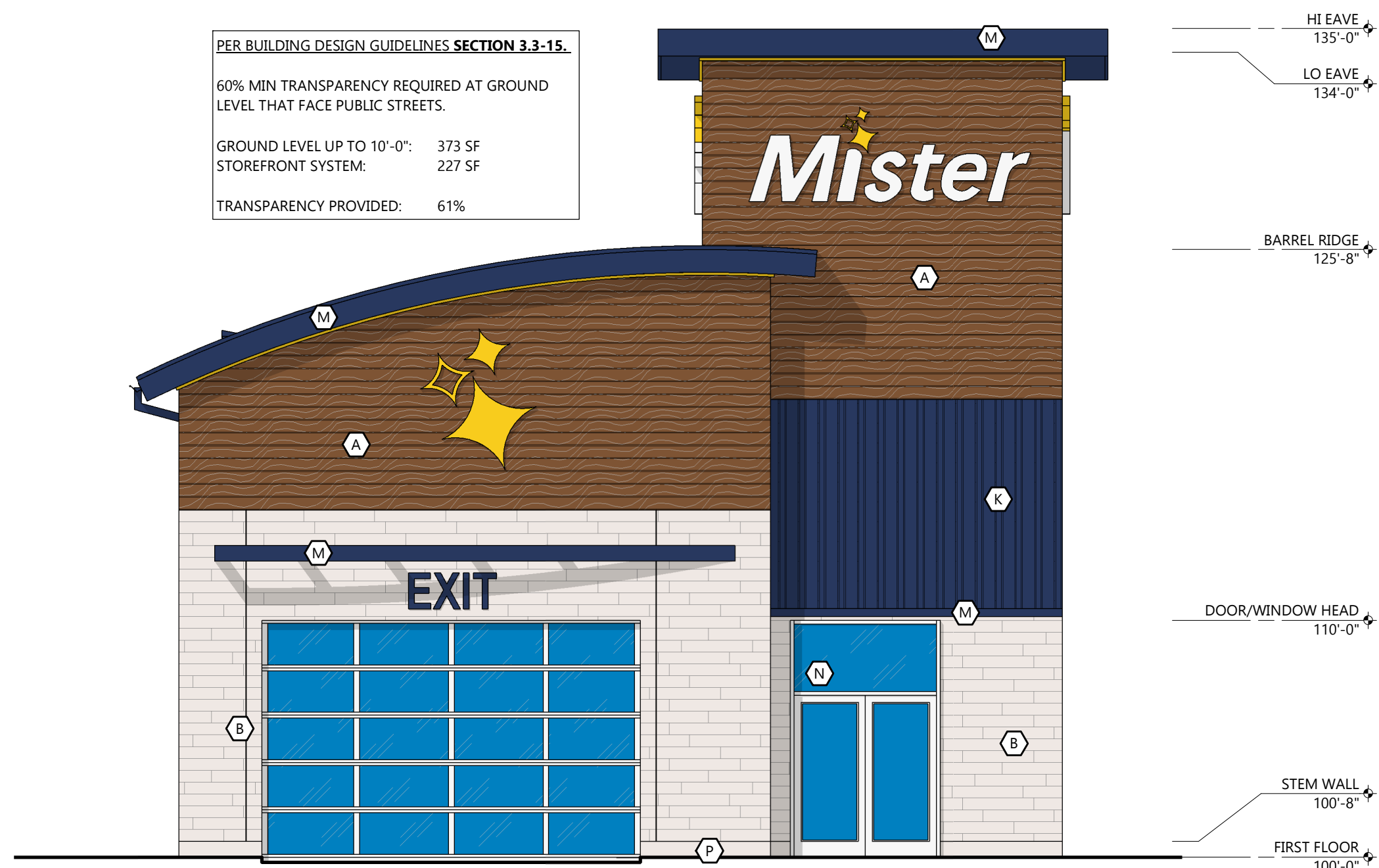
EXIT ELEVATION (WEST - SANTA ROSA AVE) SCALE: 3/16" = 1'-0"
