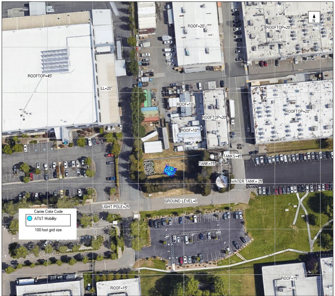
Figure 1: Antenna Locations
