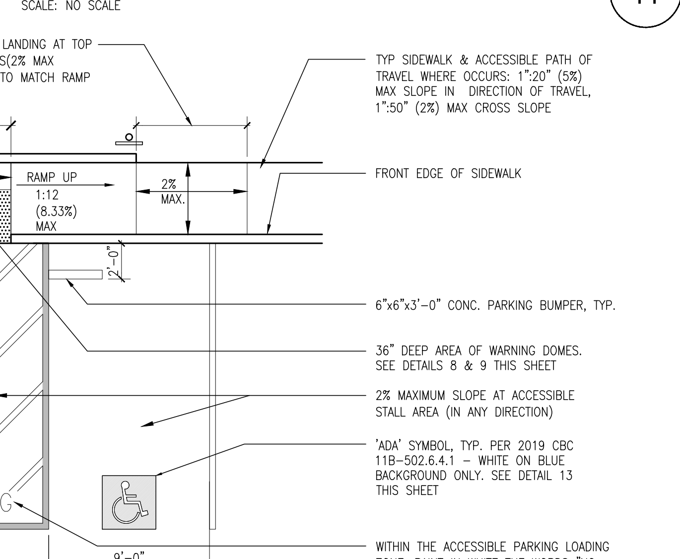
DOUBLE ACCESSIBLE STALLS SCALE: 3/16" = 1' - 0"
