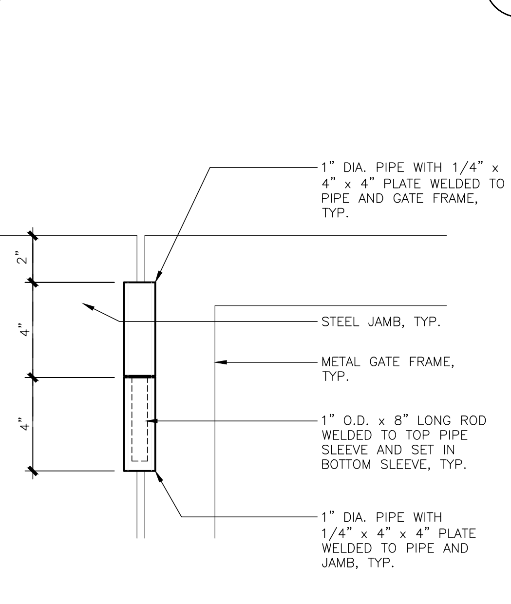
HINGE ELEVATION, TYP. SCALE: 3" = 1'-0"
