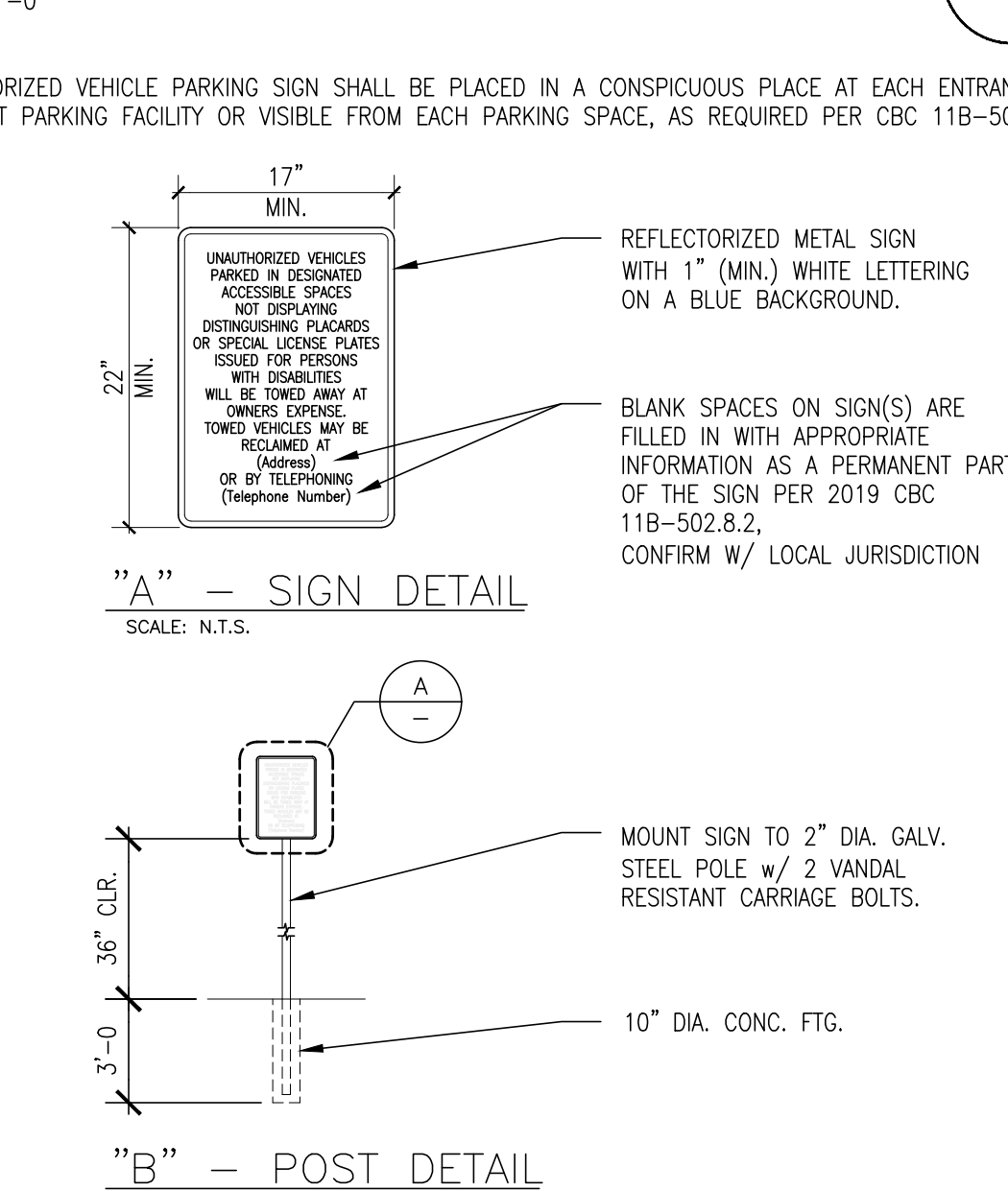
SITE ENTRY ACCESSIBLE SIGN SCALE: 3/16" = 1'-0"
