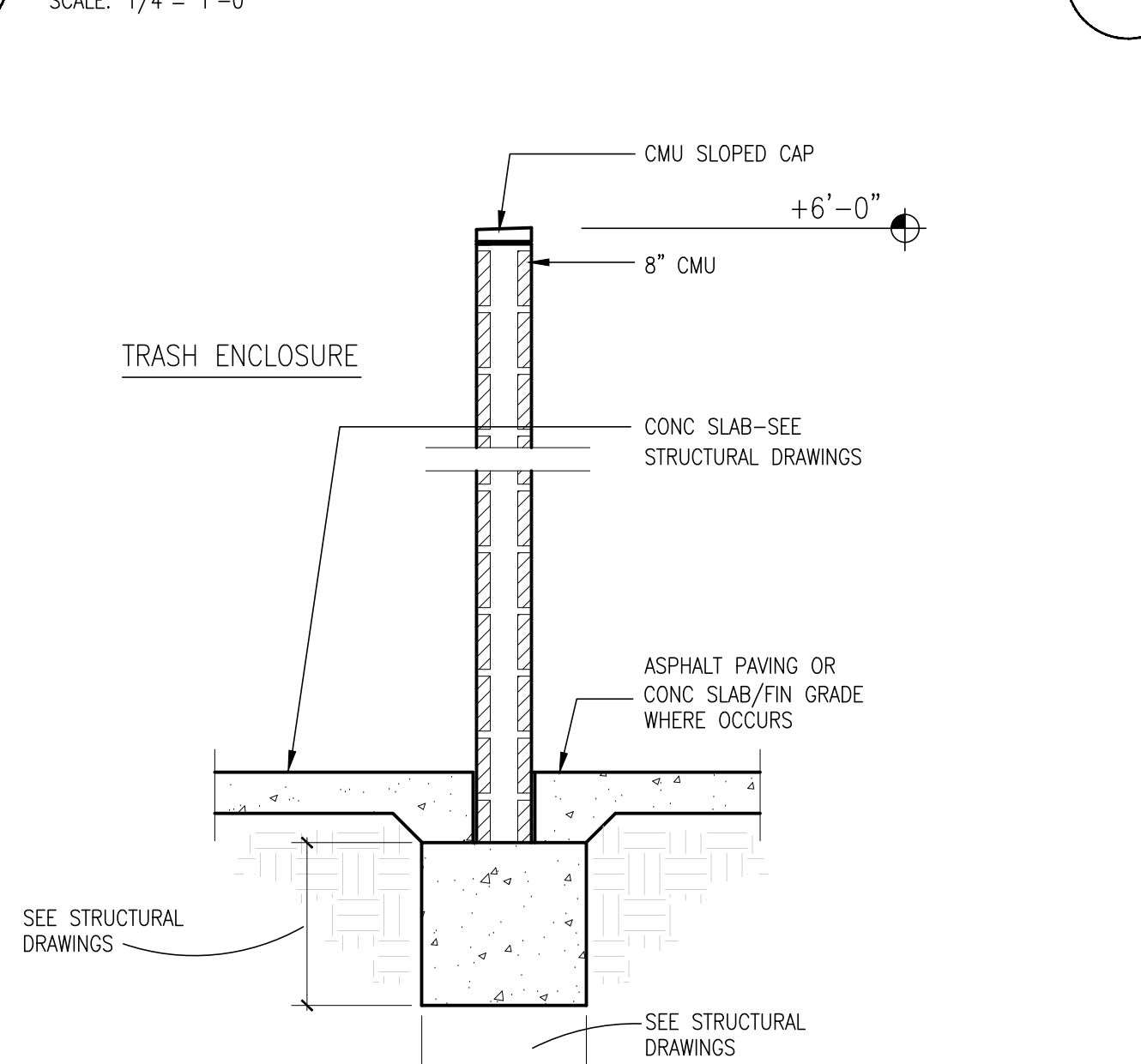
TRASH ENCLOSURE WALL SECTION SCALE: 1/2" = 1'-0"
