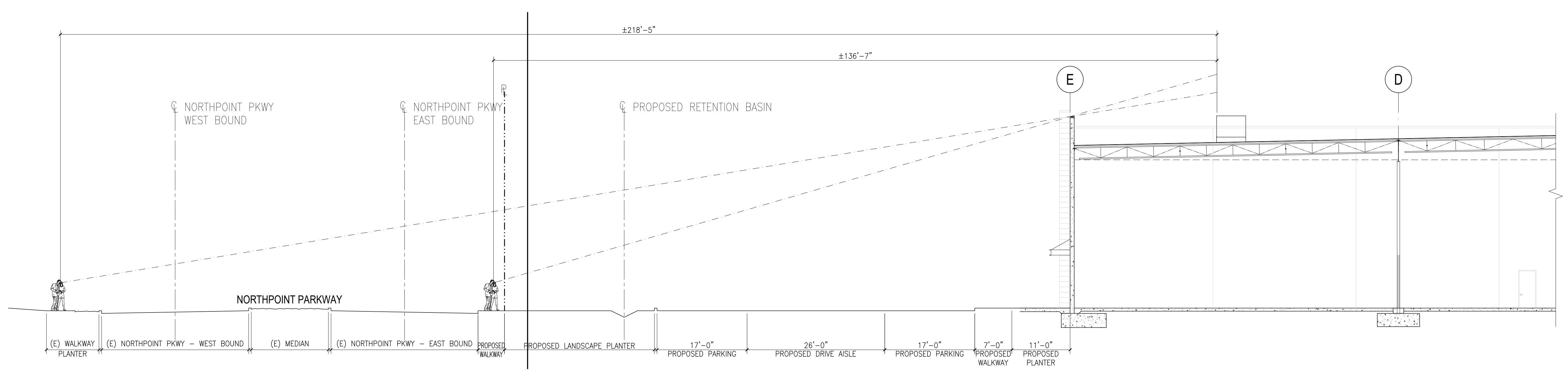
LINE OF SIGHT SECTION @ NORTHPOINT PARKWAY 3 SCALE: 1" = 10'-0"
