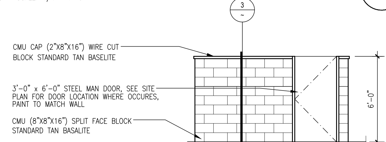
DUMPSTER ELEVATIONS SCALE: 1/4" = 1'-0"
