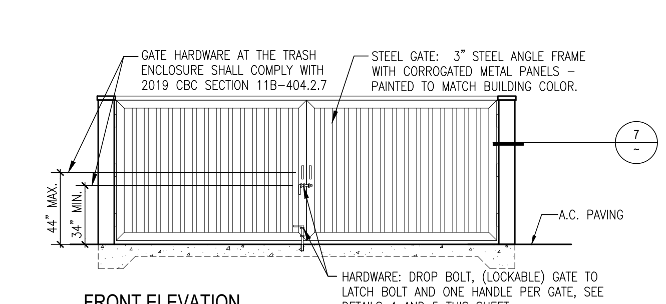
DUMPSTER ELEVATIONS SCALE: 1/4" = 1'-0"
