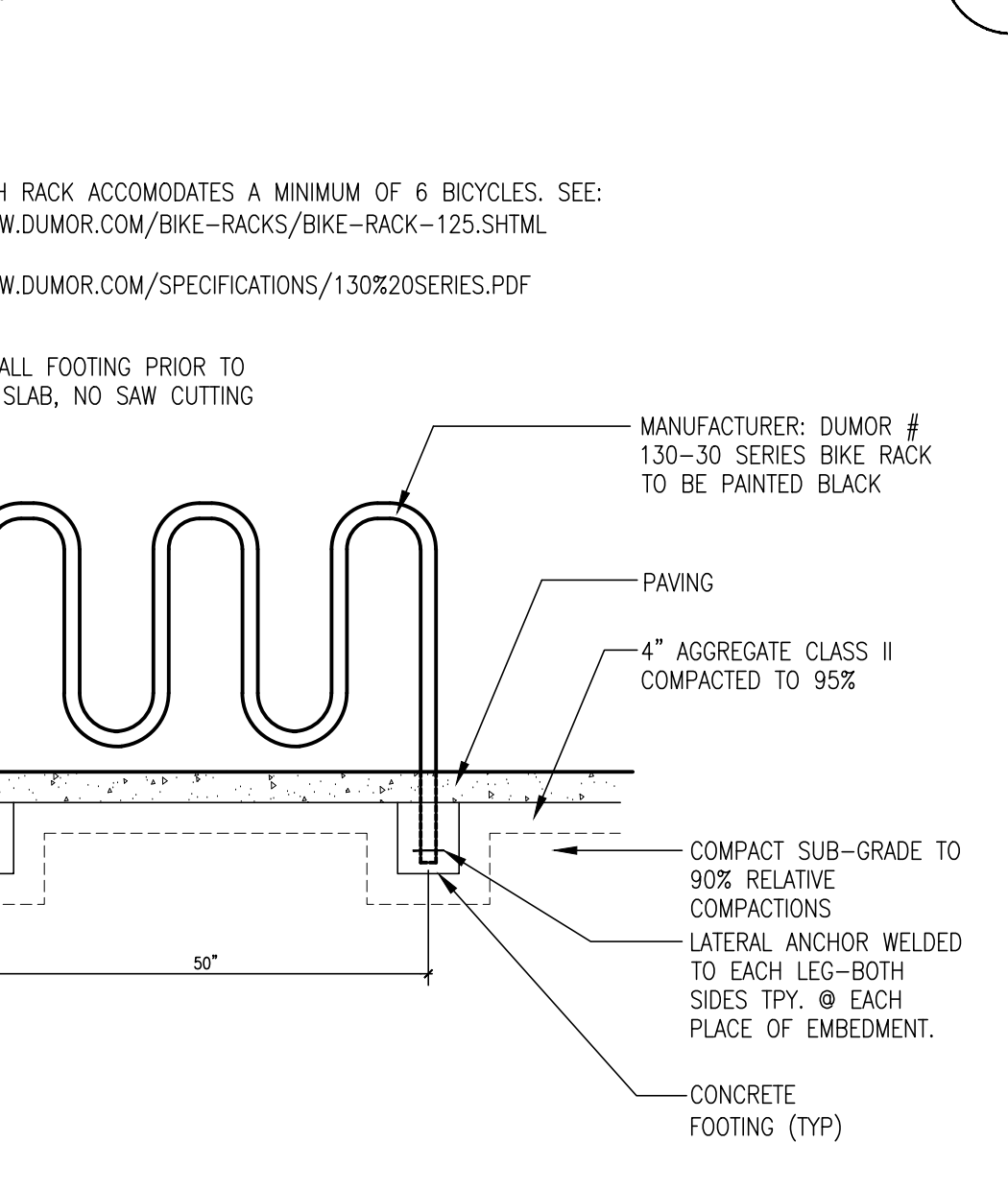
BIKE RACK SCALE: 1/2" = 1'-0"
