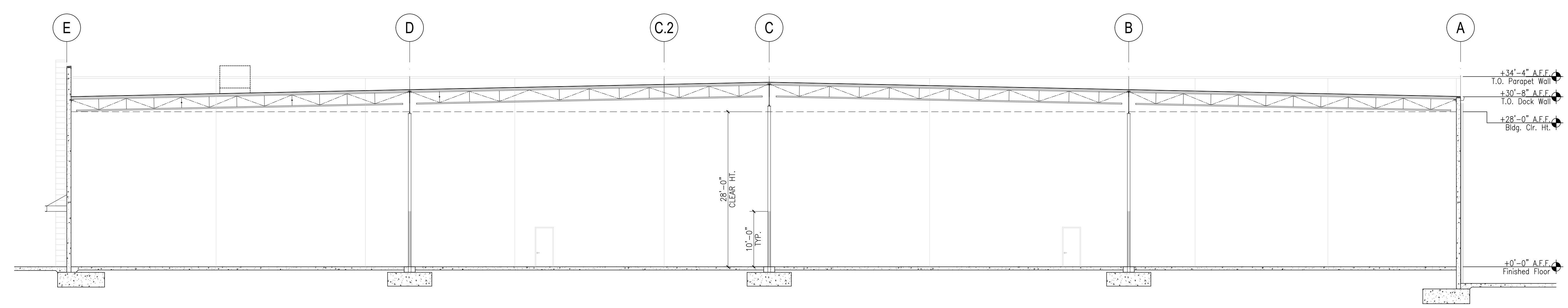
PRELIMINARY BUILDING SECTION 2 SCALE: 1" = 10'-0"
