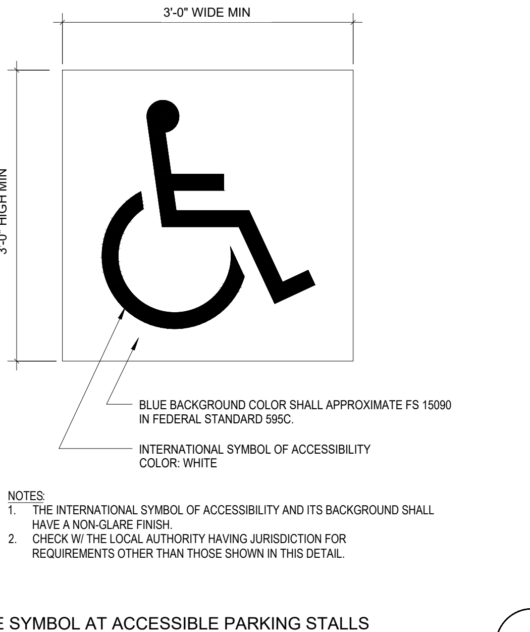
ACCESSIBLE SYMBOL AT ACCESSIBLE PARKING STALLS SCALE: 1" = 1'-0"
