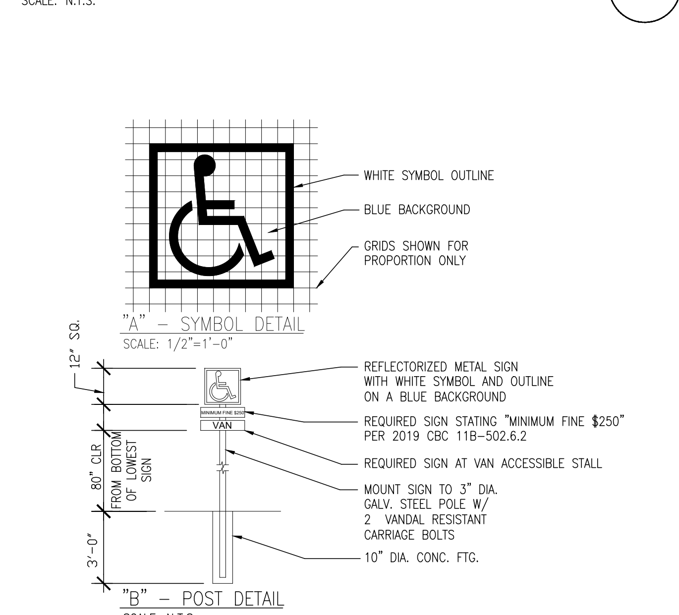
SIGN AT ACCESSIBLE PARKING STALLS SCALE: NO SCALE
