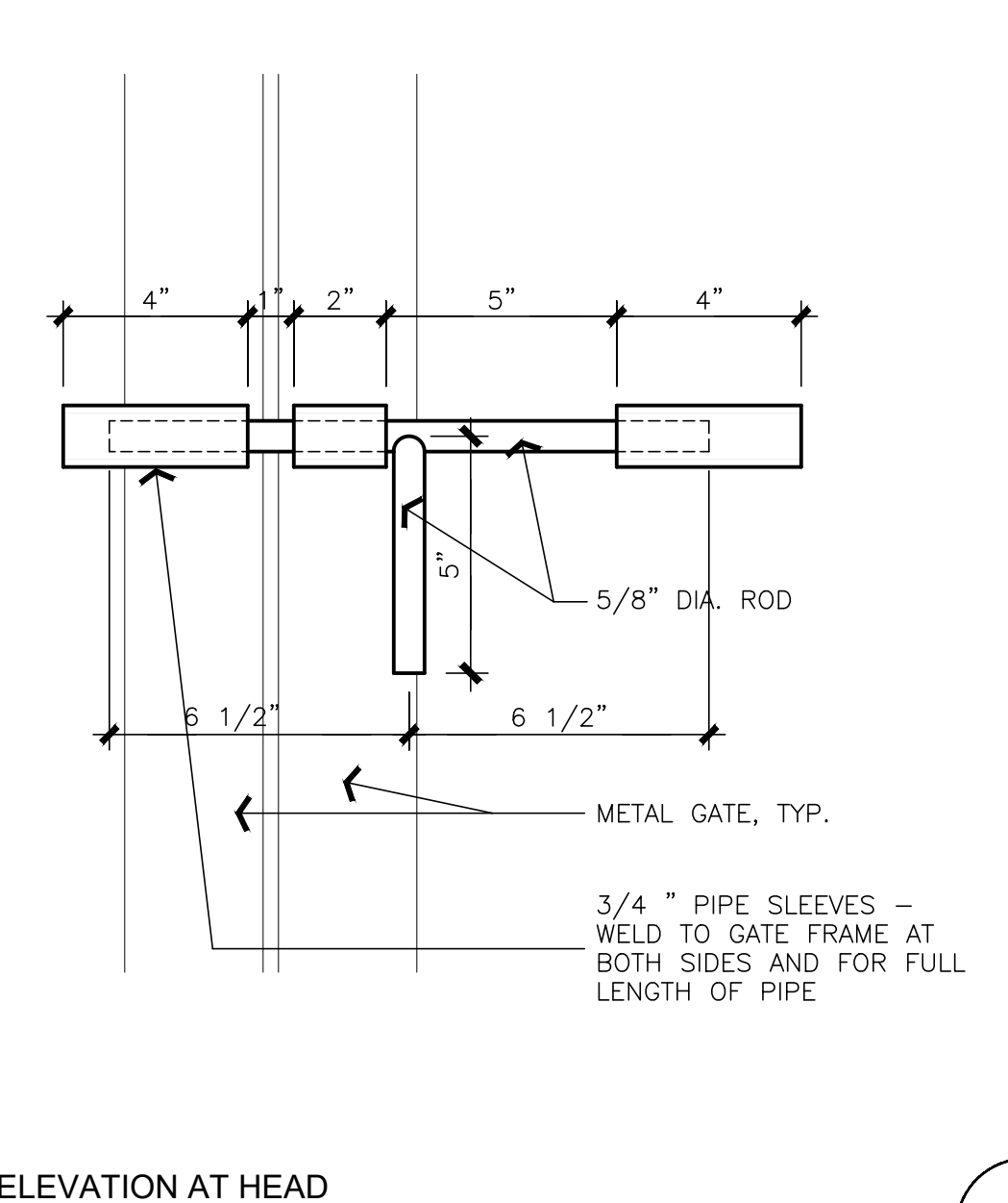
SIDE BOLT ELEVATION AT HEAD SCALE: 3" = 1'-0"
